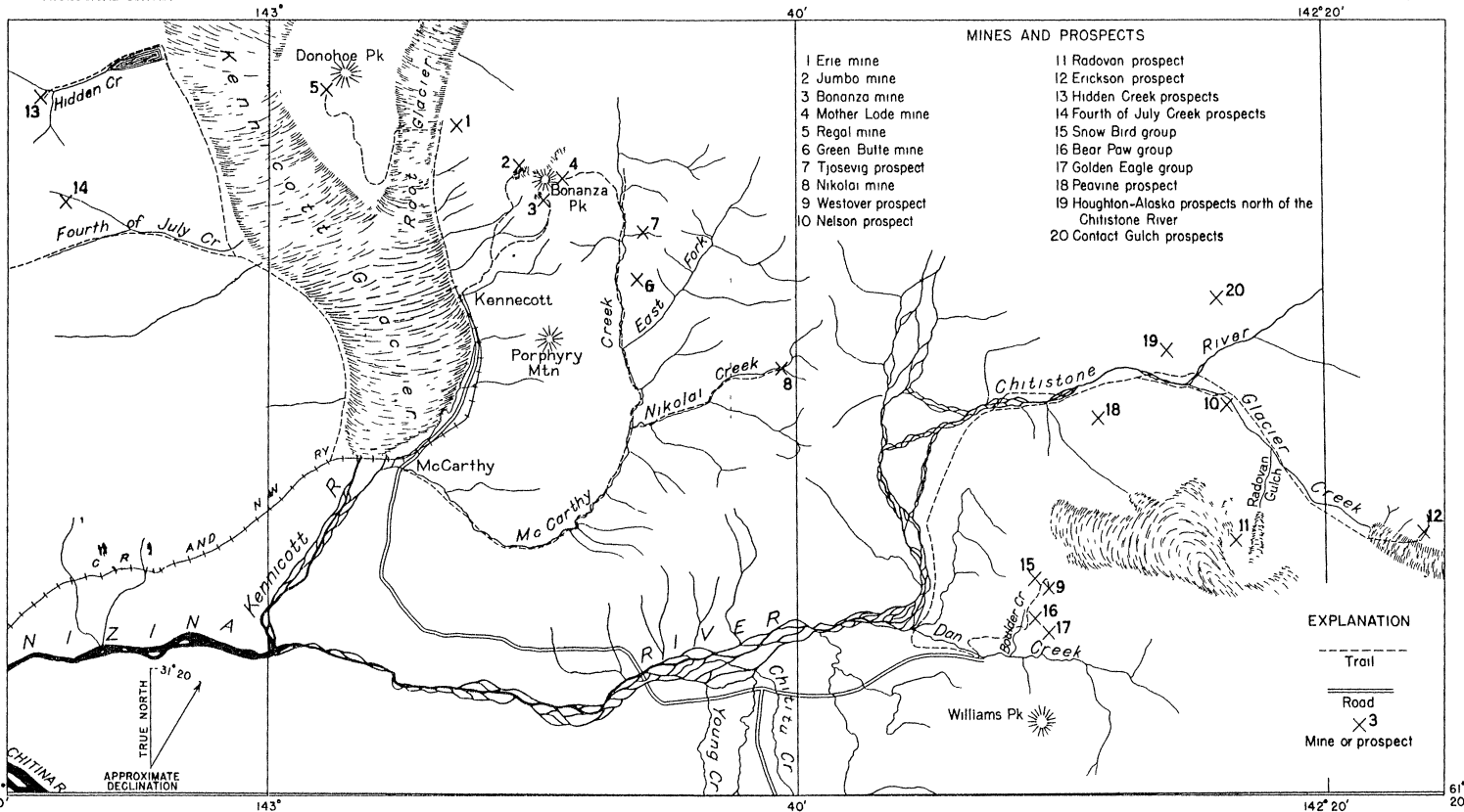
SKETCH MAP SHOWING LOCATION OF COPPER DEPOSITS OF THE NIZINA DISTRICT, ALASKA
