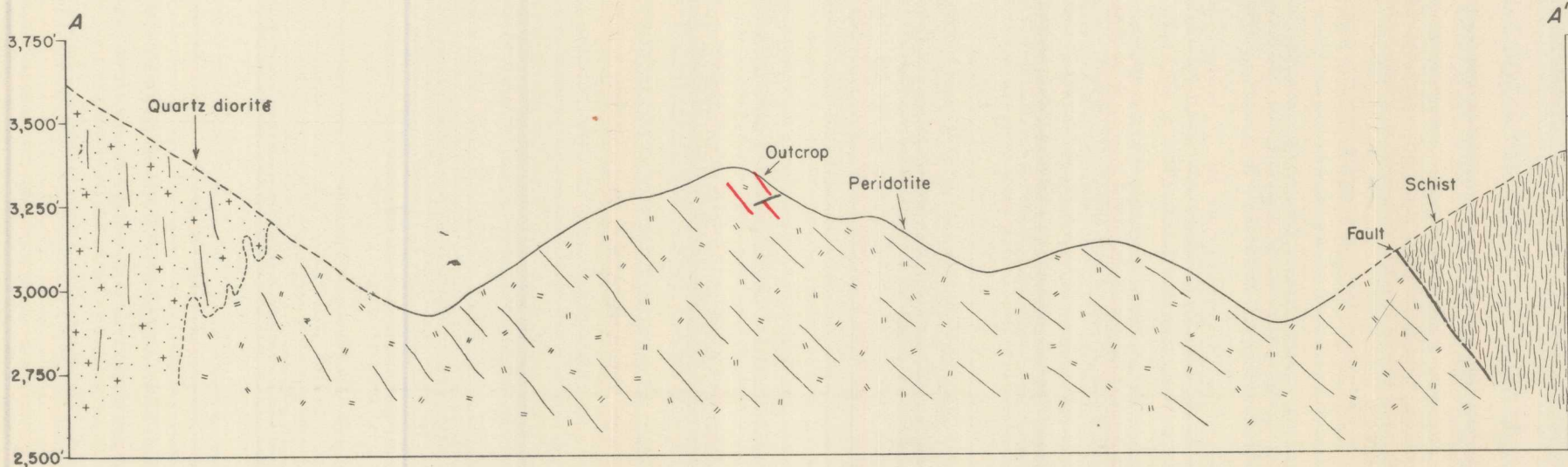
GEOLOGIC MAP AND SECTION OF THE SEIAD CREEK CHROMITE DEPOSIT, SISKIYOU COUNTY, CALIFORNIA
