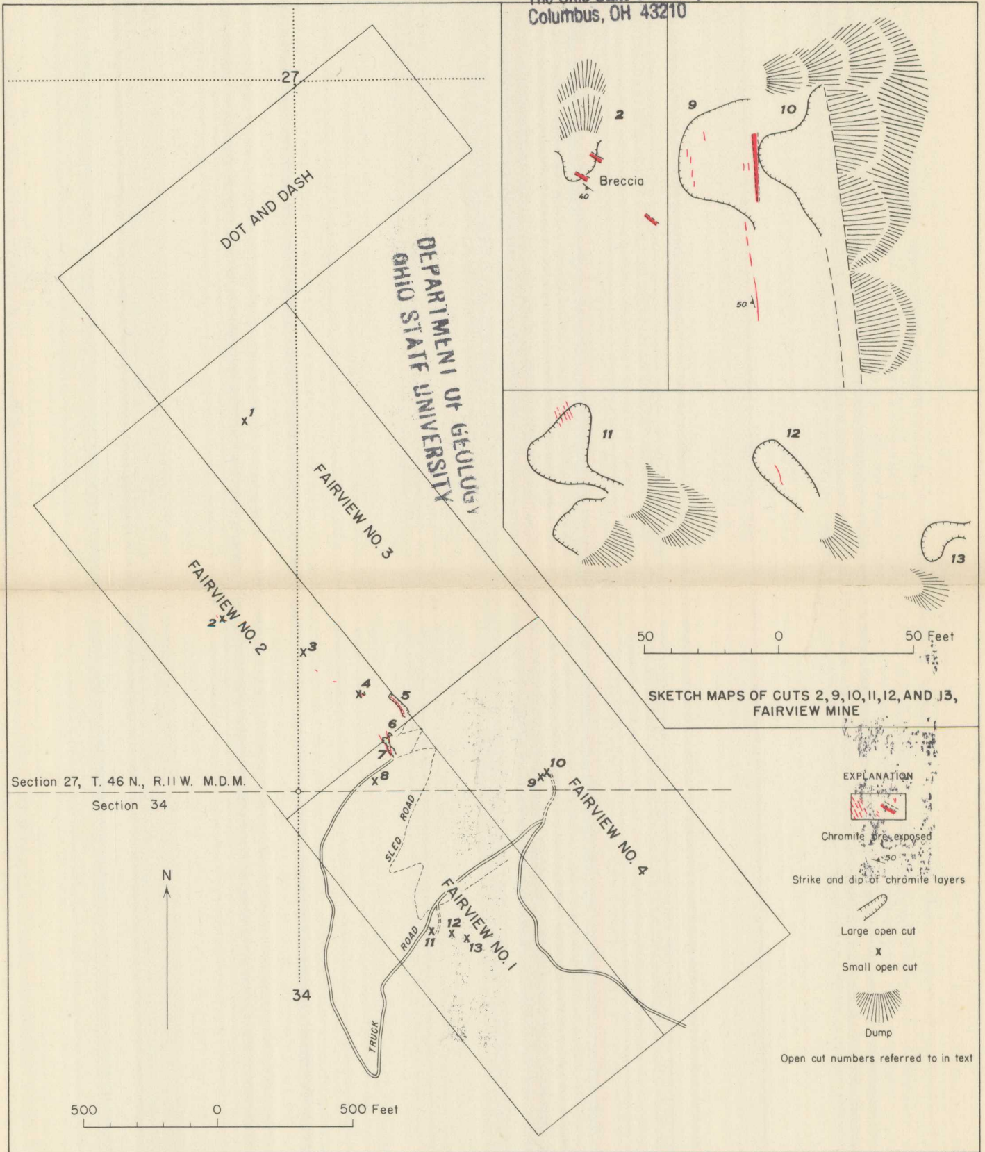
MAP OF THE FAIRVIEW GROUP OF CHROMITE CLAIMS, SISKIYOU COUNTY, CALIFORNIA, WITH SKETCH MAPS OF CUTS 2, 9, 10, 11, 12, AND 13
