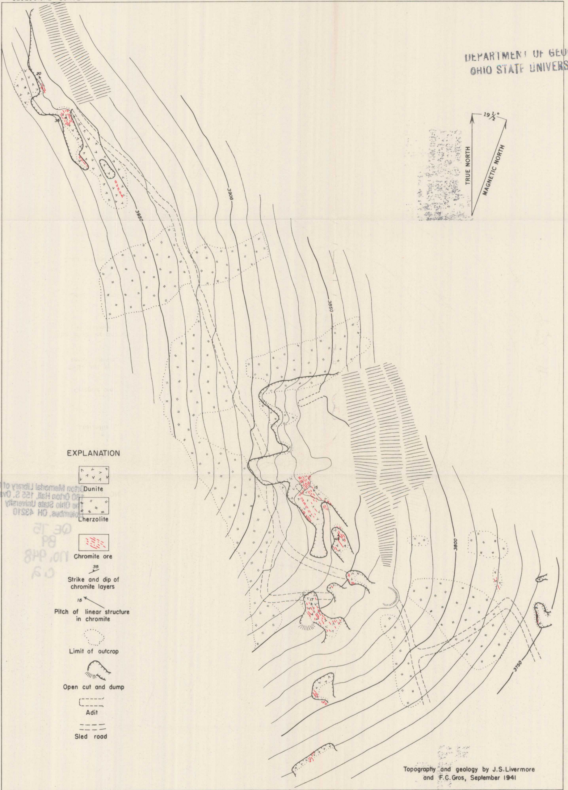
GEOLOGIC OUTCROP MAP OF THE VETA GRANDE CHROMITE DEPOSIT, SISKIYOU COUNTY, CALIFORNIA
