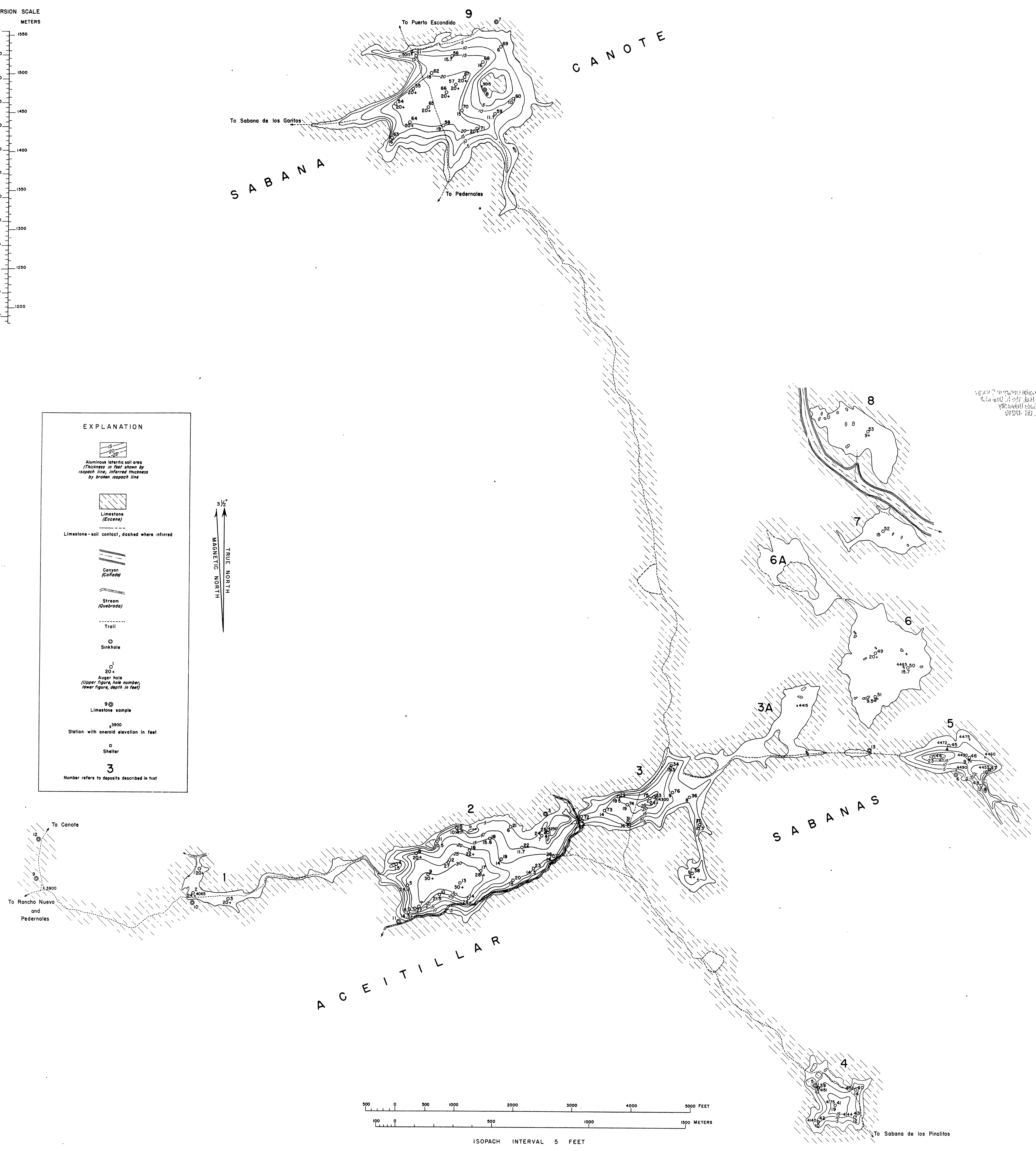
ISOPACH MAP OF ALUMINOUS LATERITIC SOIL DEPOSITS OF ACEITILLAR AREA, SIERRA DE BAHORUCO, DOMINICAN REPUBLIC
