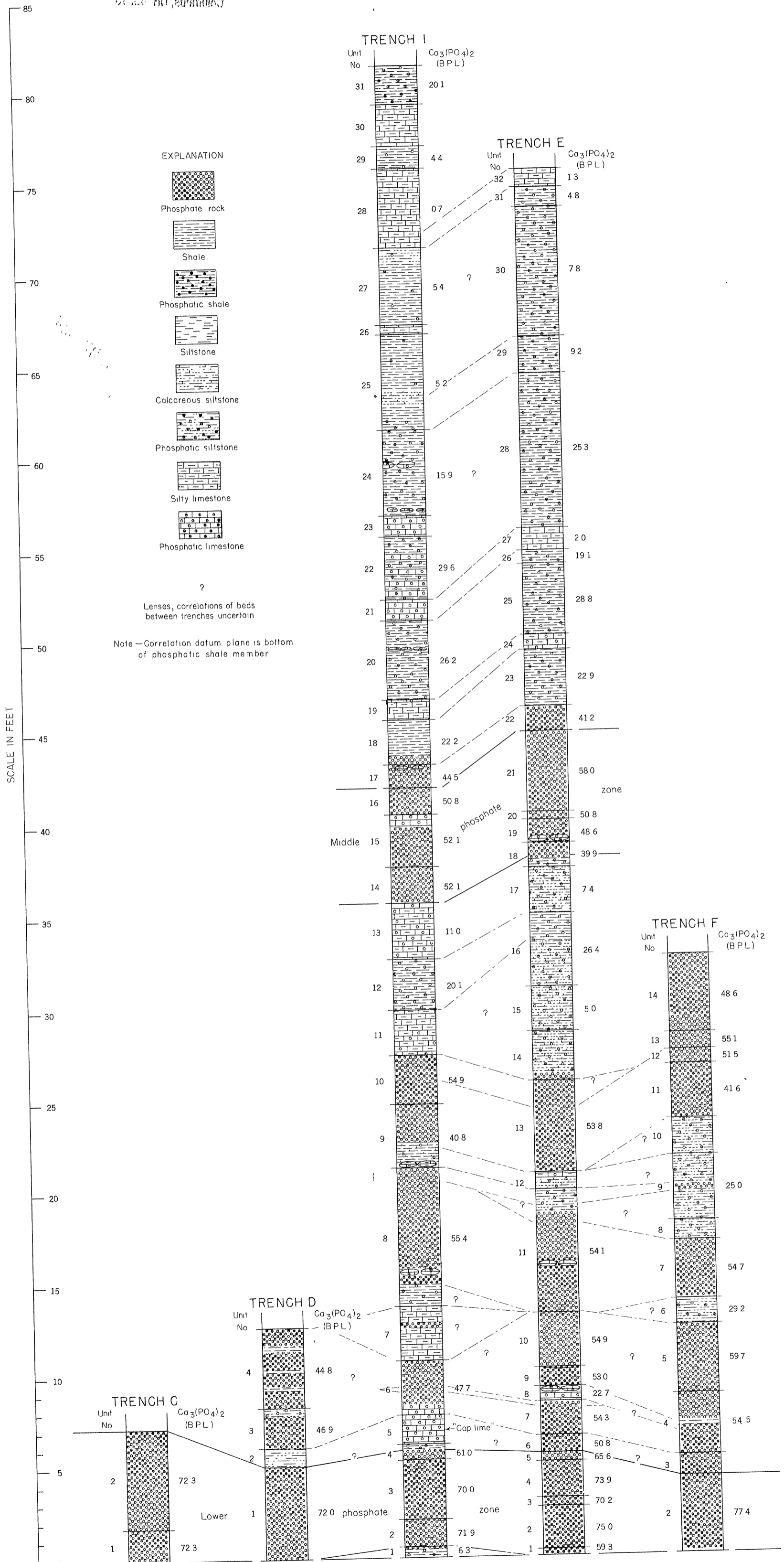
COLUMNAR SECTIONS, LOWER PART OF PHOSPHATIC SHALE MEMBER, PHOSPHORIA FORMATION, DEER CREEK - WELLS CANYON AREA, IDAHO
