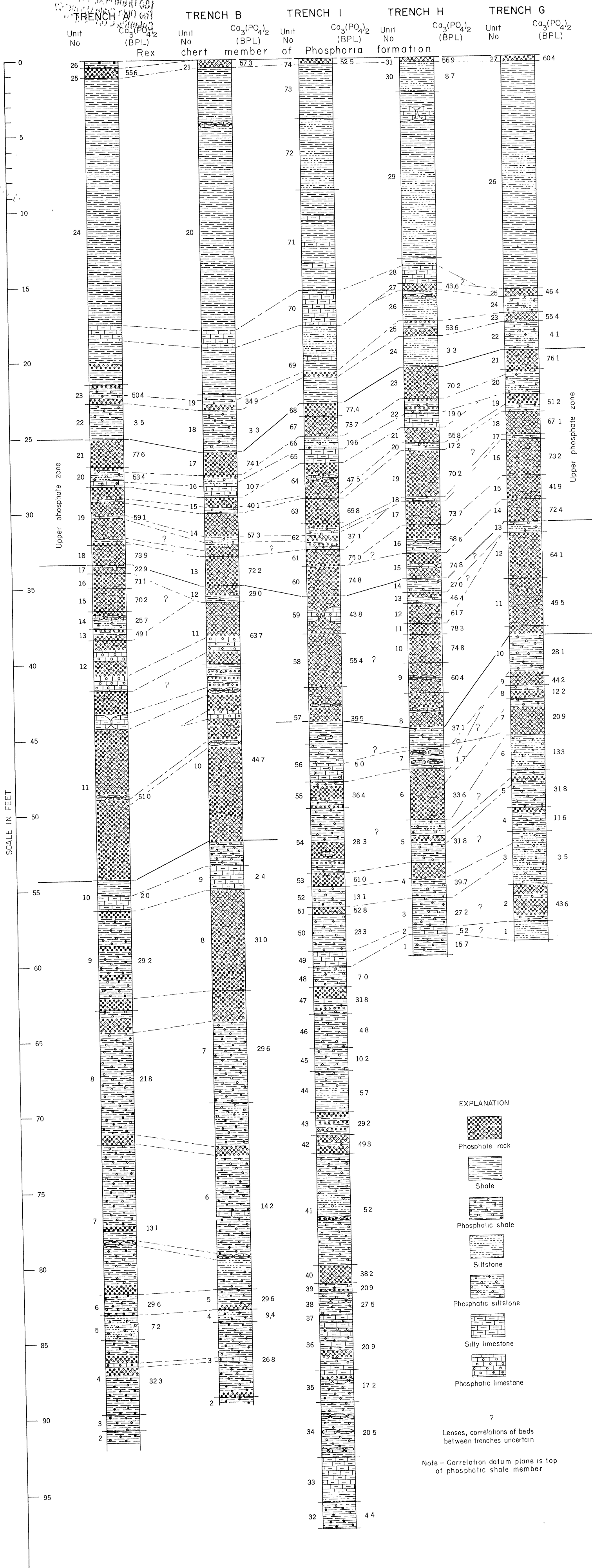
COLUMNAR SECTIONS, UPPER PART OF PHOSPHATIC SHALE MEMBER, PHOSPHORIA FORMATION, DEER CREEK - WELLS CANYON AREA, IDAHO
