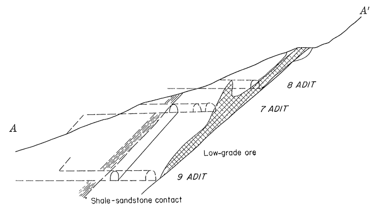
PROFILE AND SECTION THROUGH SOUTH ORE BODY
