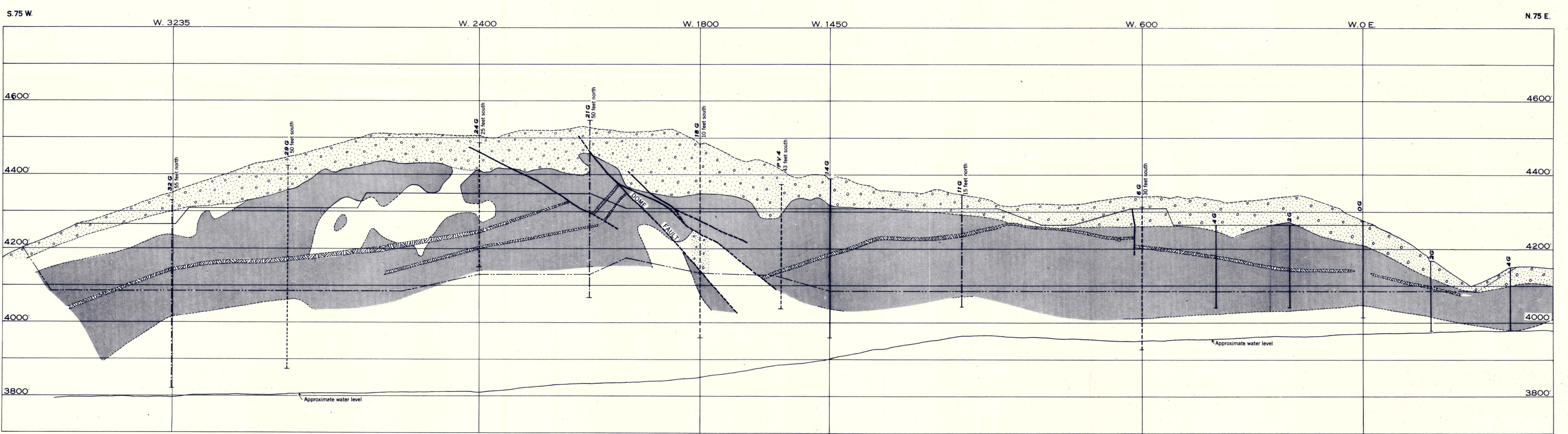
STRUCTURE SECTIONS OF THE CASTLE DOME MINE, GILA COUNTY, ARIZONA
