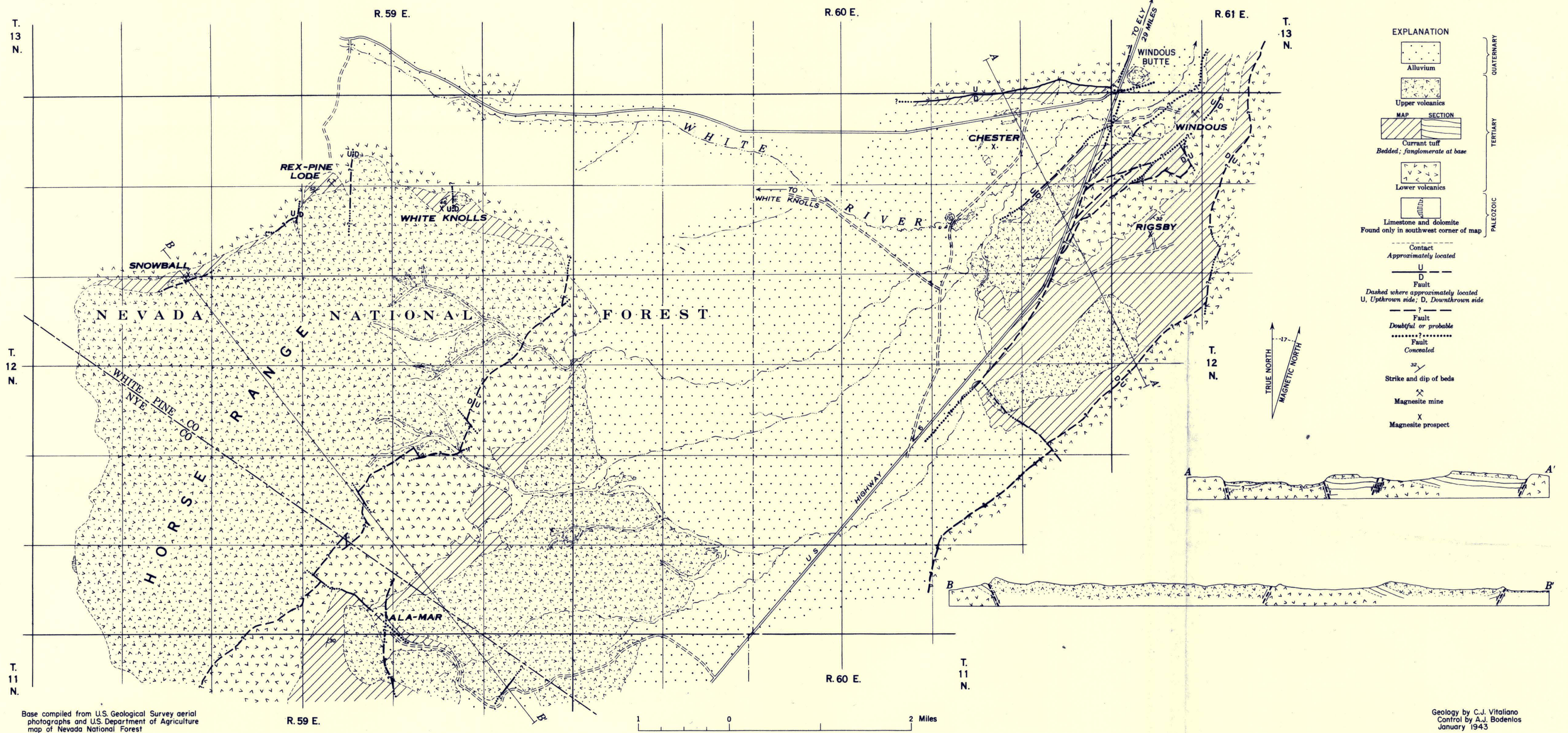
GEOLOGIC MAP AND SECTIONS SHOWING THE DISTRIBUTION OF THE MAGNESITE DEPOSITS IN THE CURRANT CREEK DISTRICT, WHITE PINE AND NYE COUNTIES, NEVADA
