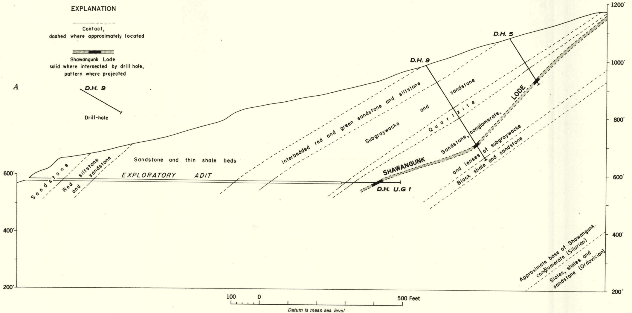
GENERALIZED CROSS SECTION THROUGH EXPLORATORY ADIT SHAWANGUNK MINE SULLIVAN COUNTY NEW YORK
