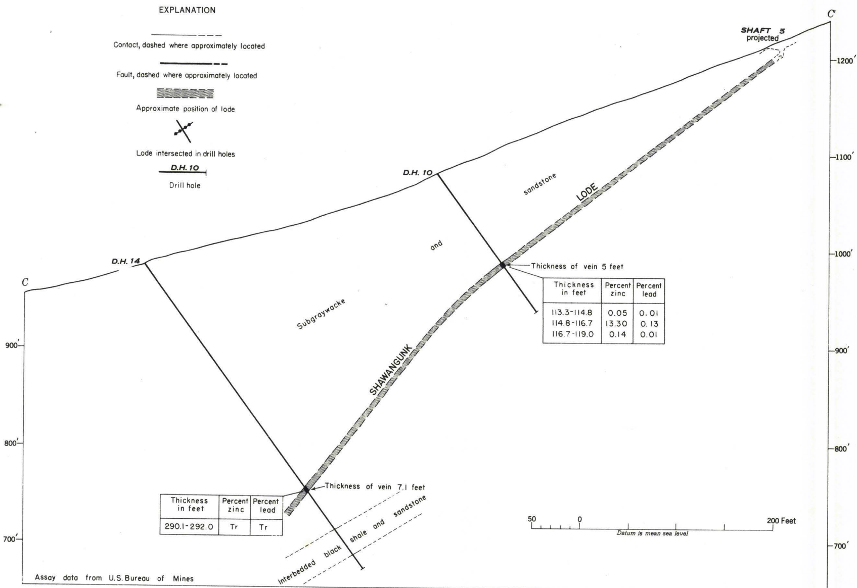
CROSS SECTIONS THROUGH SHAWANGUNK LODE AND DRILL HOLES, SHAWANGUNK MINE, SULLIVAN COUNTY, NEW YORK.
