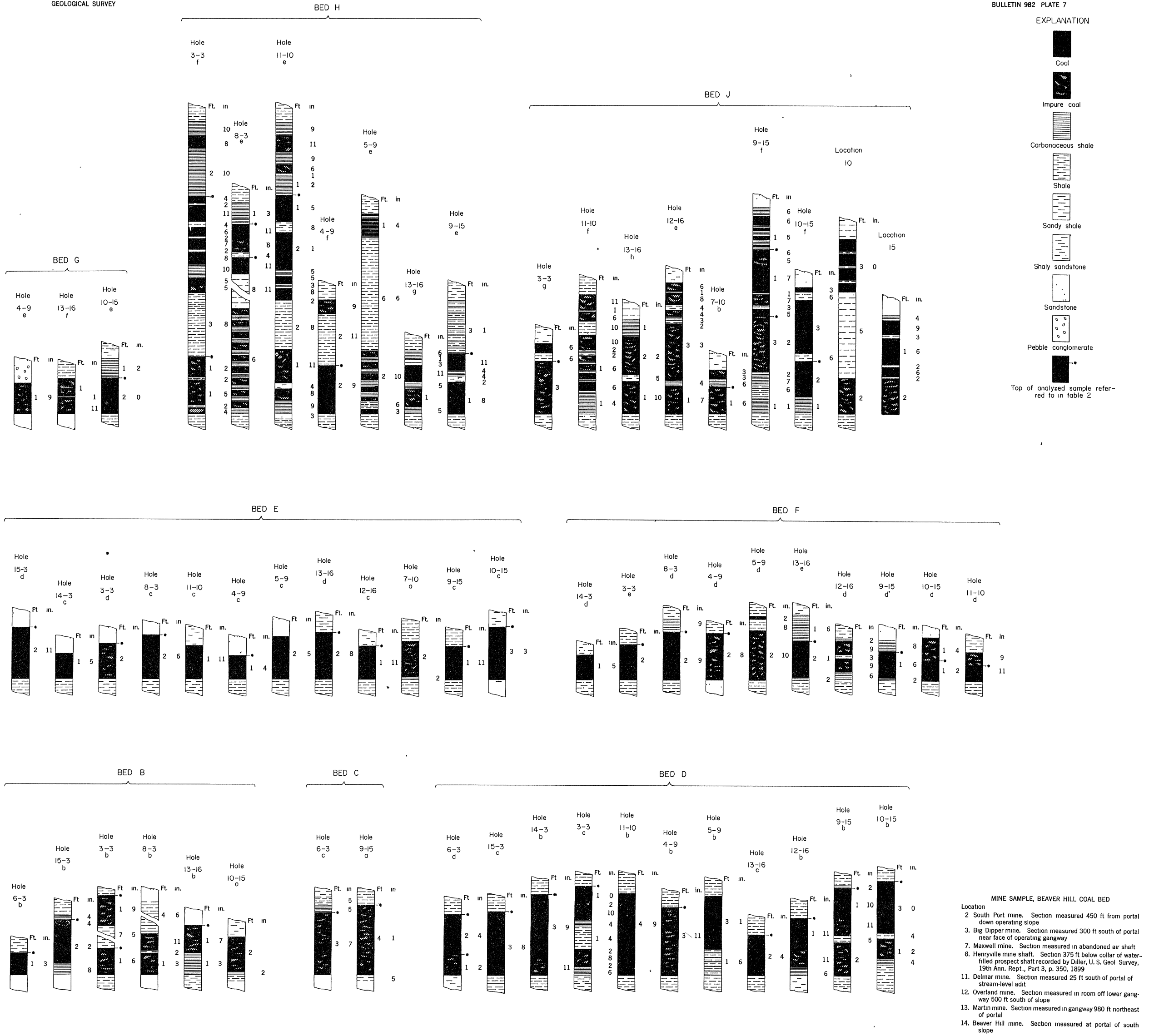
BEAVER HILL COAL BED 0 10 Feet Vertical scale DETAILED COLUMNAR SECTIONS OF COAL BEDS IN TPS. 26 AND 27 S., R. 13 W., COOS COUNTY, OREGON
