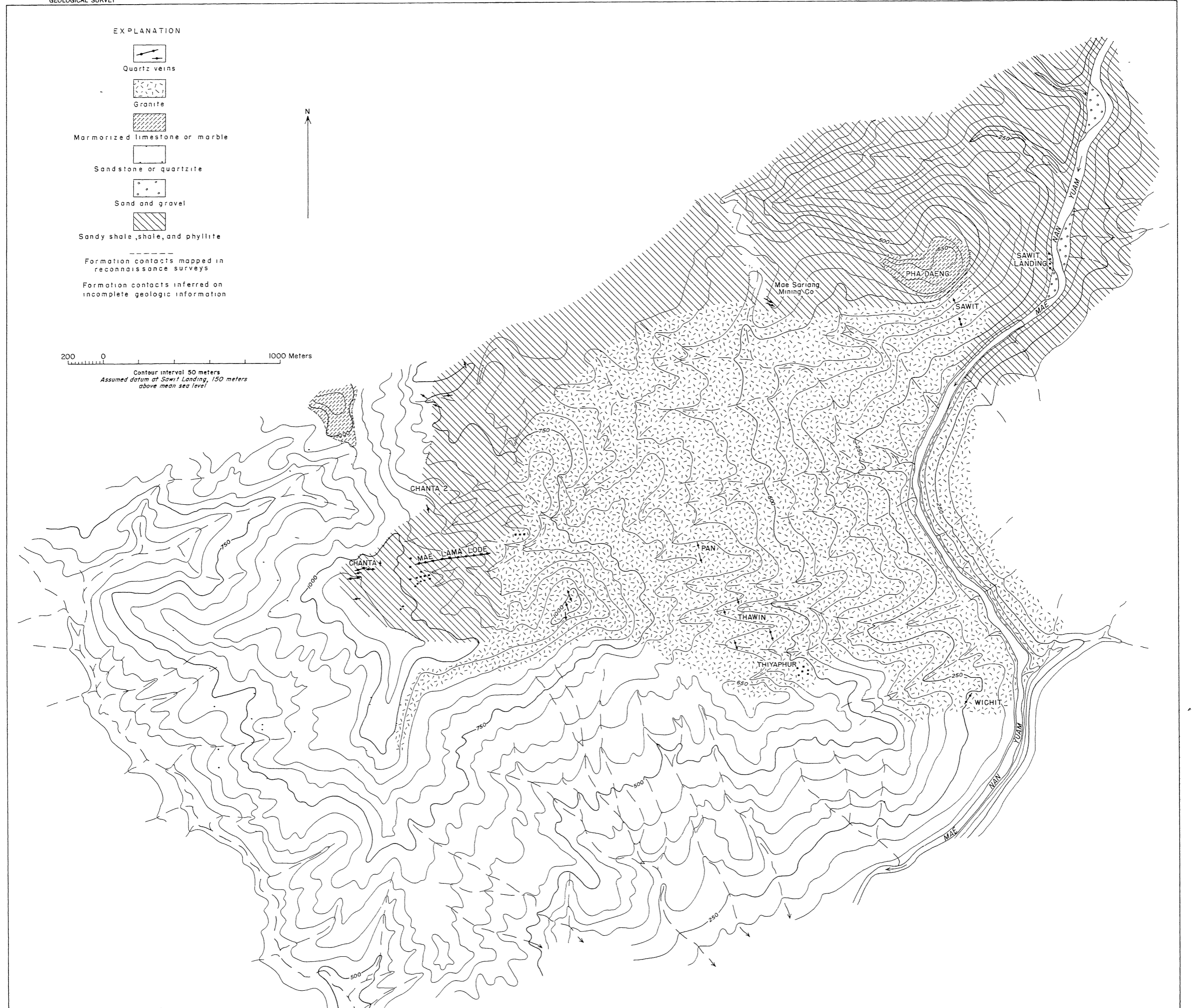
GEOLOGIC SKETCH MAP OF THE MAE SARIANG TUNGSTEN DISTRICT CHANGWAT MAE HONG SON
