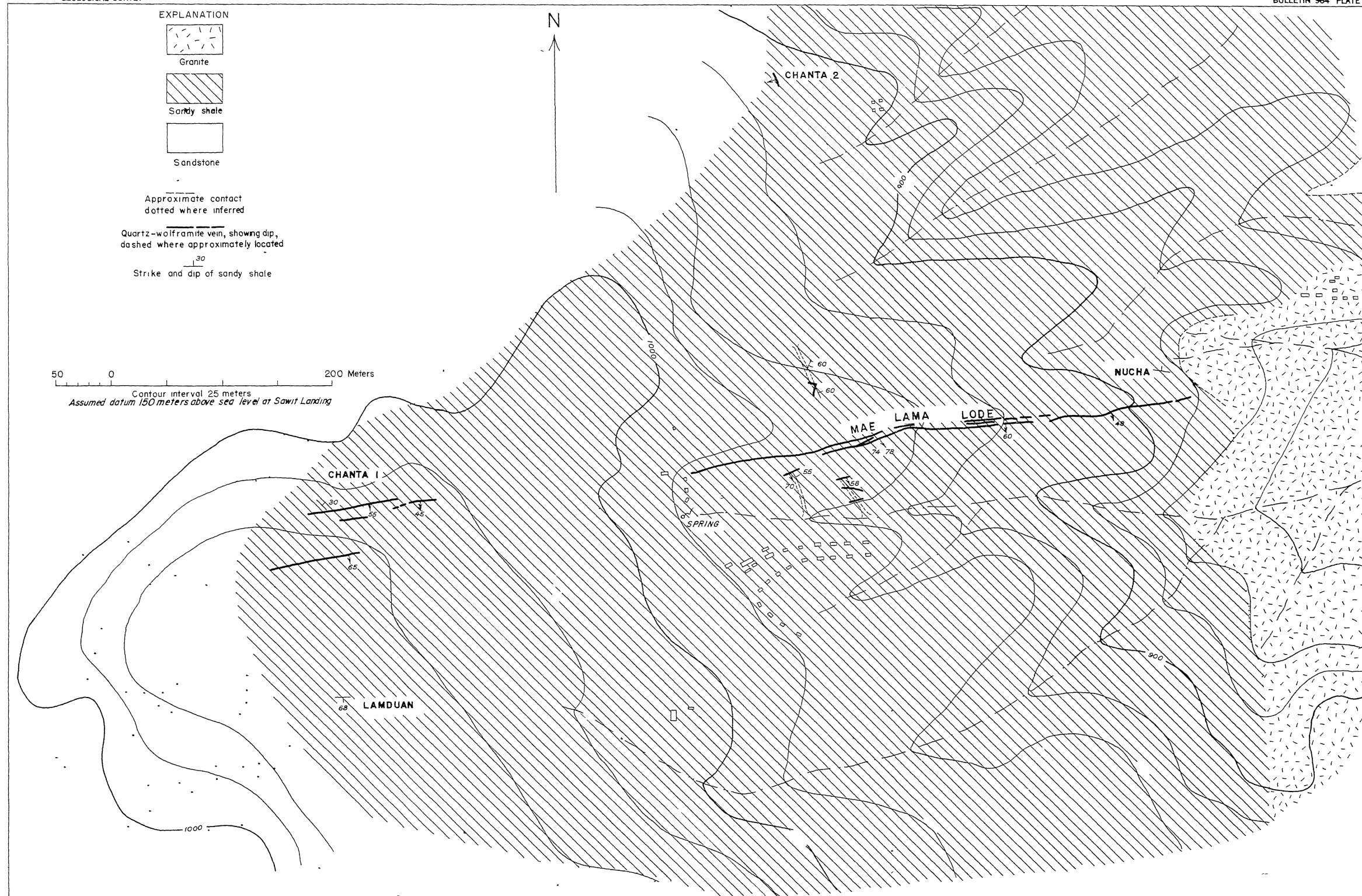
GEOLOGIC SKETCH MAP OF THE MAE LAMA TUNGSTEN LODE AND ADJACENT LEASES, MAE SARIANG DISTRICT, CHANGWAT MAE HONG SON
