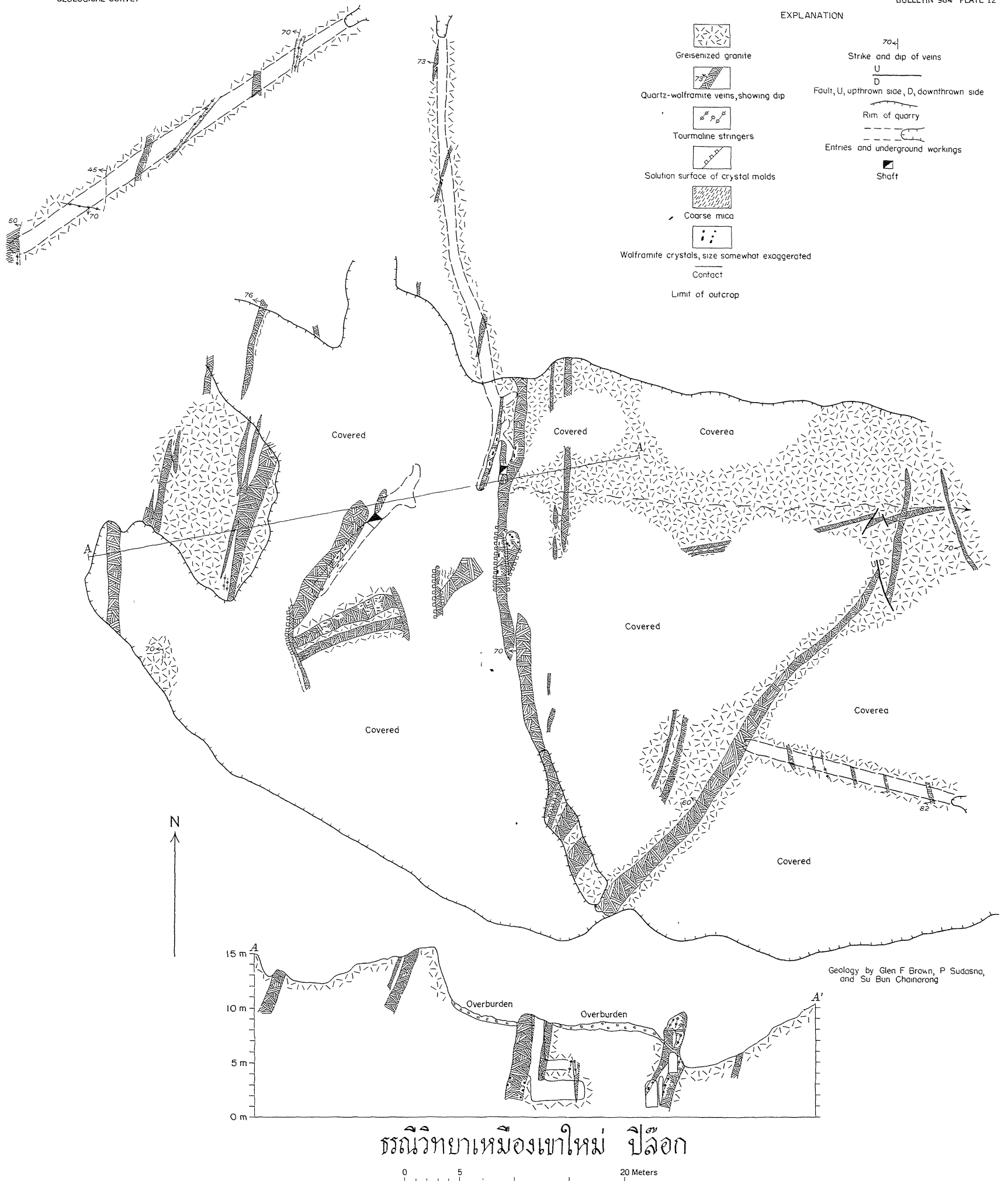
GEOLOGIC SKETCH MAP OF KHAO MAI TUNGSTEN-TIN MINE, PILOK DISTRICT
