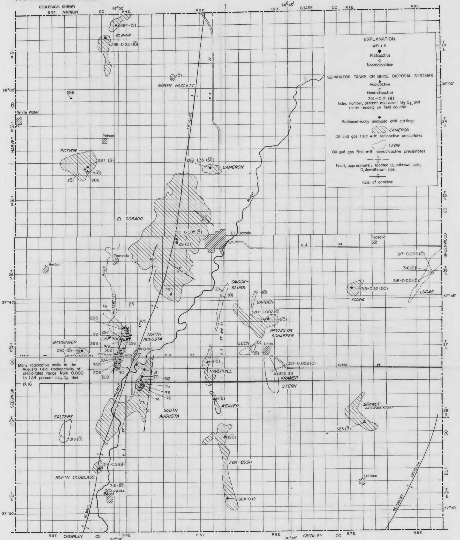
LOCATION OF RADIUM-BEARING PRECIPITATES, BUTLER COUNTY, KANSAS
