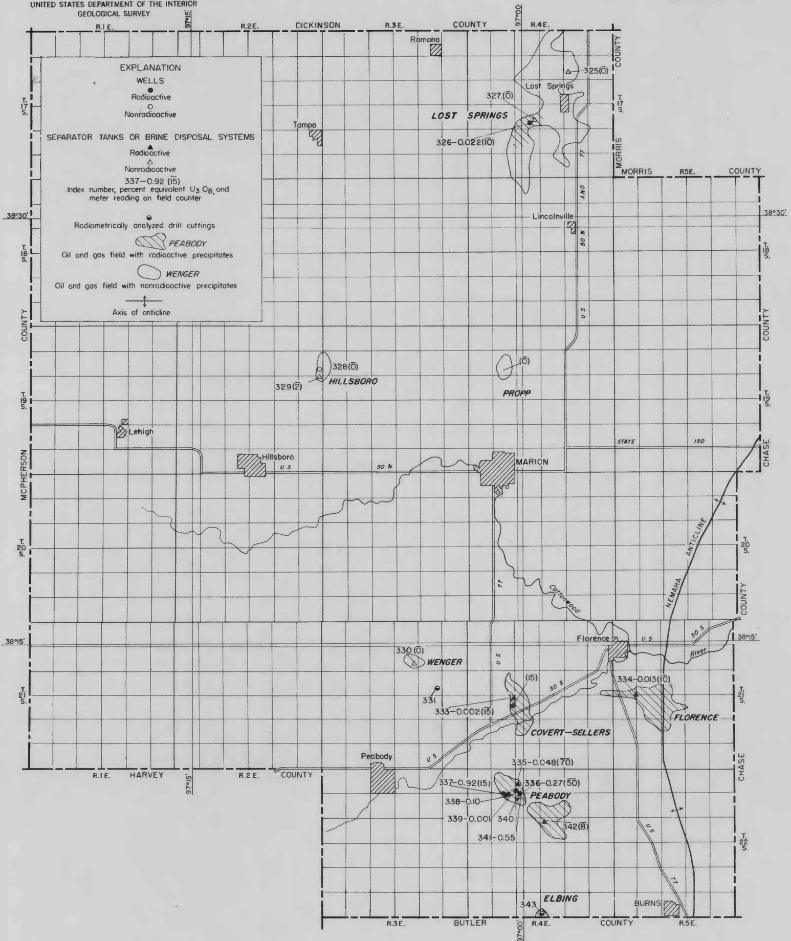
LOCATION OF RADIUM-BEARING PRECIPITATES, MARION COUNTY, KANSAS
