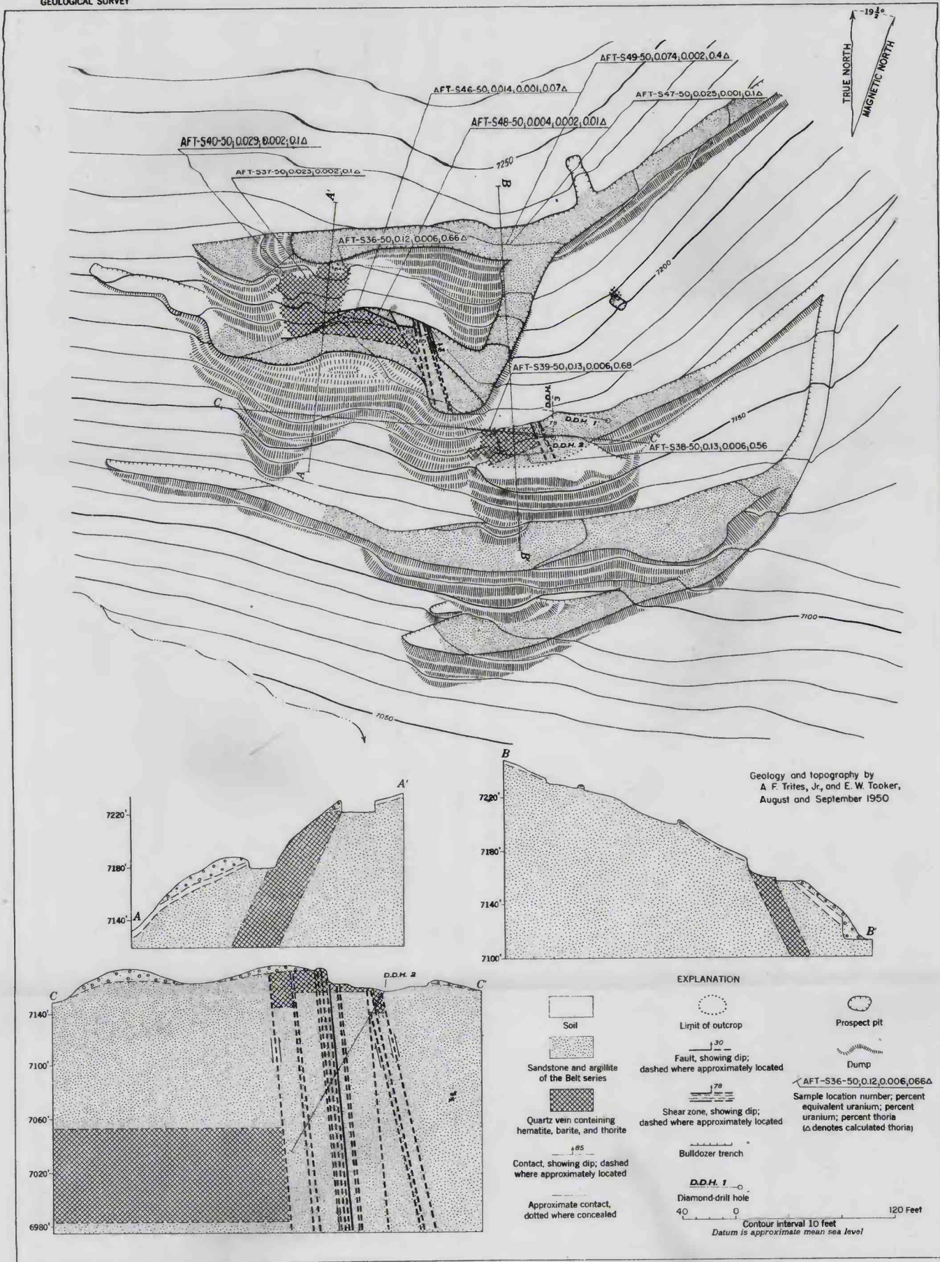
GEOLOGIC MAP AND SECTIONS OF THE TRAPPER NO. 4 CLAIM, BEAVERHEAD COUNTY, MONTANA
