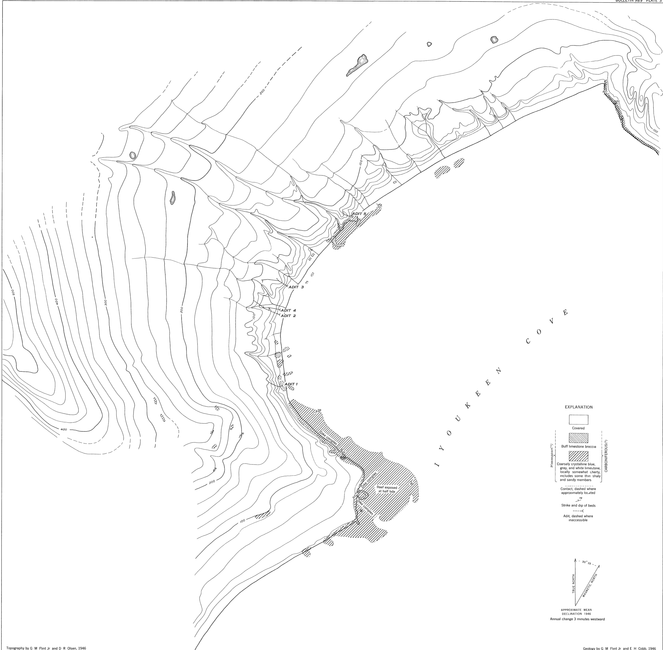
TOPOGRAPHIC AND GEOLOGIC MAP OF GYPSUM-CAMEL PROPERTY AND VICINITY, IYOUKEEN COVE, CHICHAGOF ISLAND, SOUTHEASTERN ALASKA
