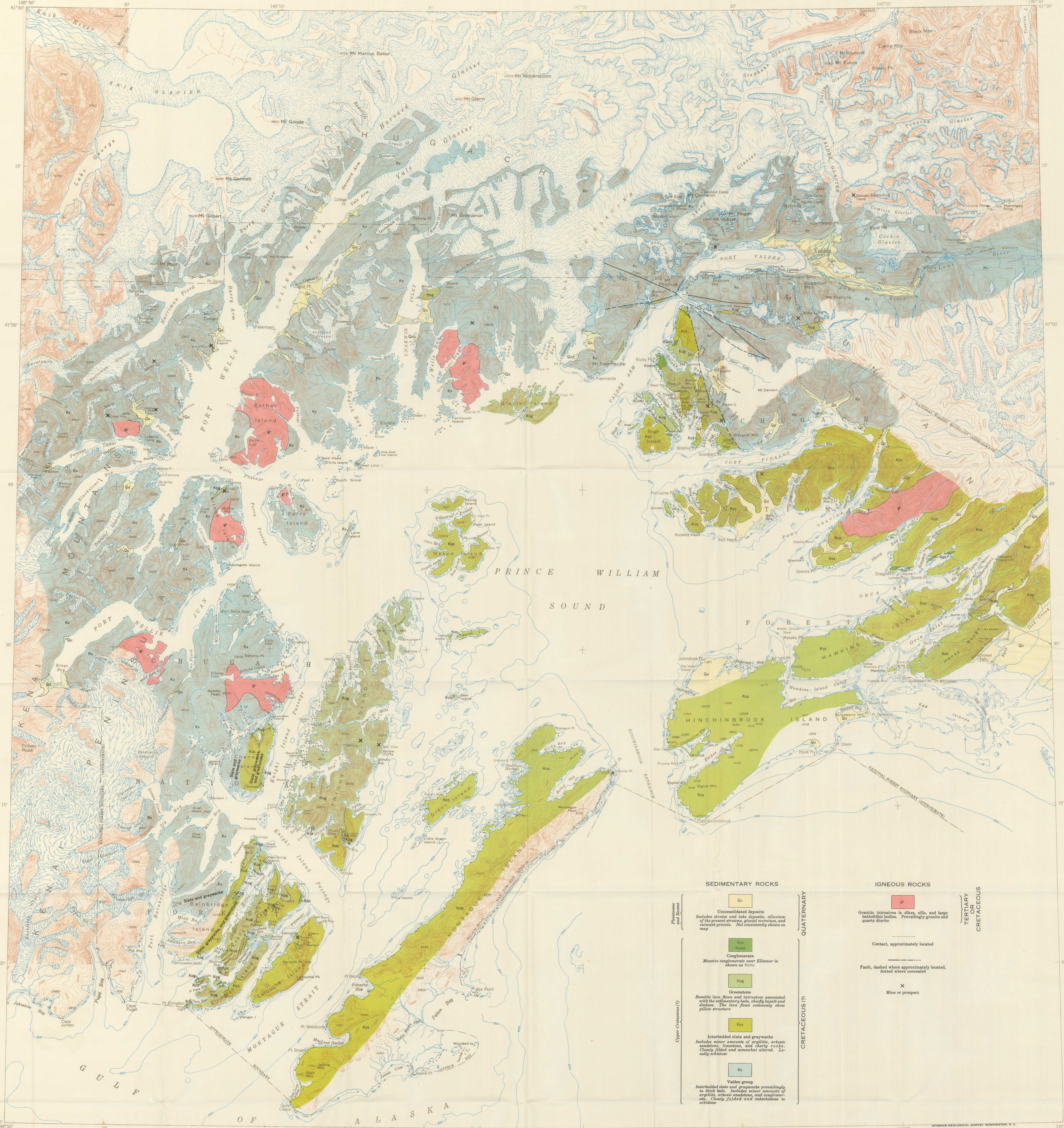
GEOLOGIC MAP OF PRINCE WILLIAM SOUND, ALASKA
