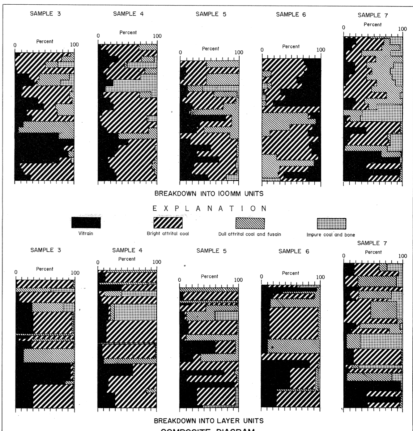
CONSTITUTION DIAGRAMS OF COAL SAMPLES FROM THE BOTTOM SPLIT MAMMOTH COAL BED
