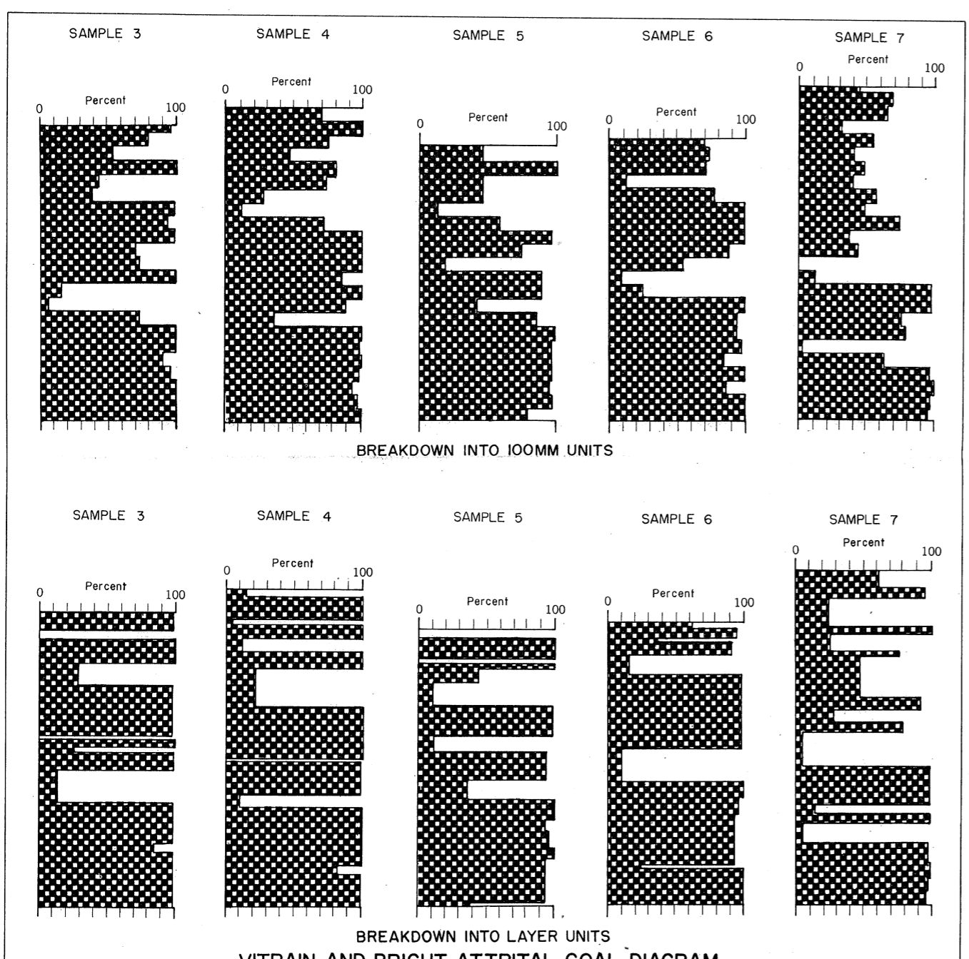
CONSTITUTION DIAGRAMS OF COAL SAMPLES FROM THE BOTTOM SPLIT MAMMOTH COAL BED
