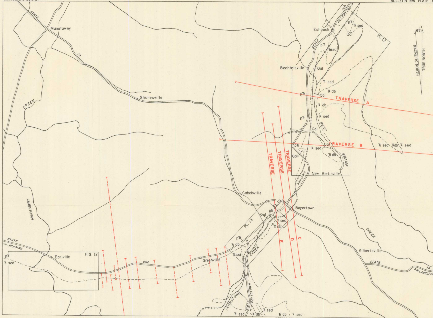
INDEX MAP SHOWING LOCATION OF DETAILED MAGNETIC AND GEOLOGIC MAPS OF BOYERTOWN AND VICINITY, PENNSYLVANIA
