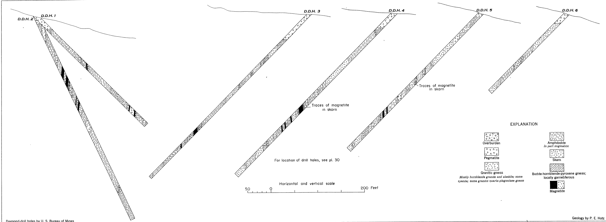
SECTIONS THROUGH DIAMOND-DRILL HOLES, CUMMINS MINE, NEW JERSEY
