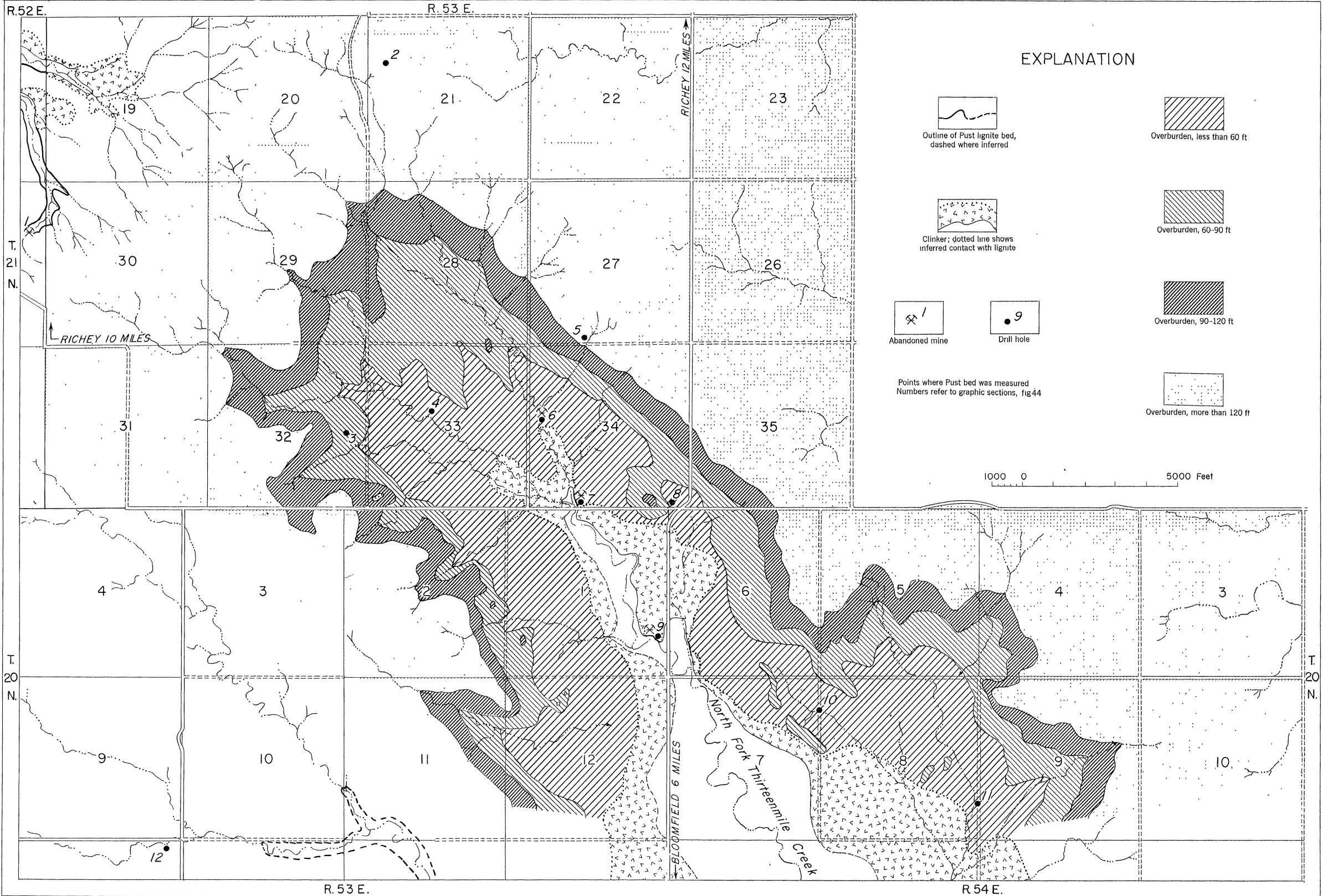
MAP OF NORTH FORK THIRTEENMILE CREEK STRIPPABLE DEPOSIT IN PUST LIGNITE BED, DAWSON COUNTY, MONTANA
