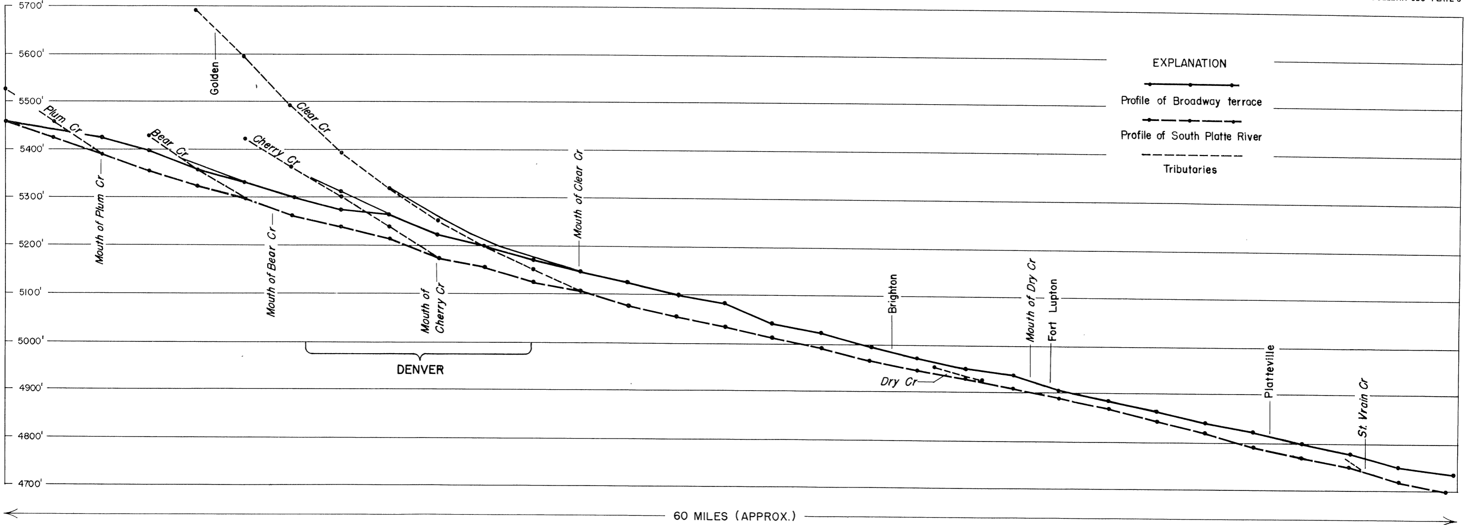
PROFILES OF SOUTH PLATTE RIVER AND BROADWAY TERRACE IN THE DENVER AREA, COLORADO
