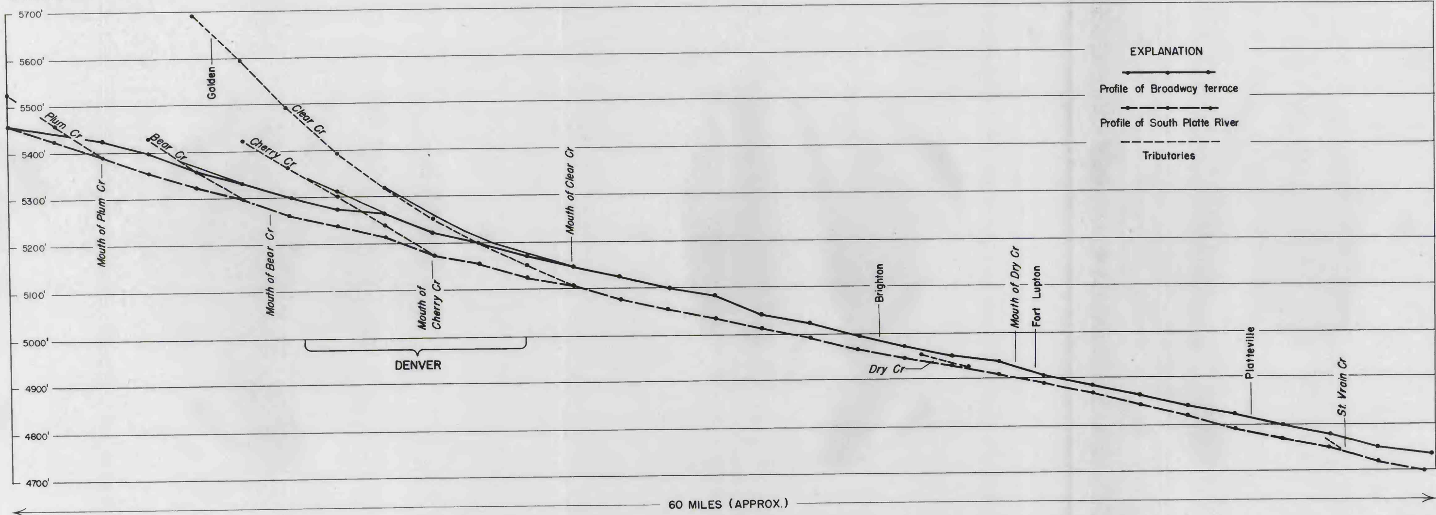
PROFILES OF SOUTH PLATTE RIVER AND BROADWAY TERRACE IN THE DENVER AREA, COLORADO
