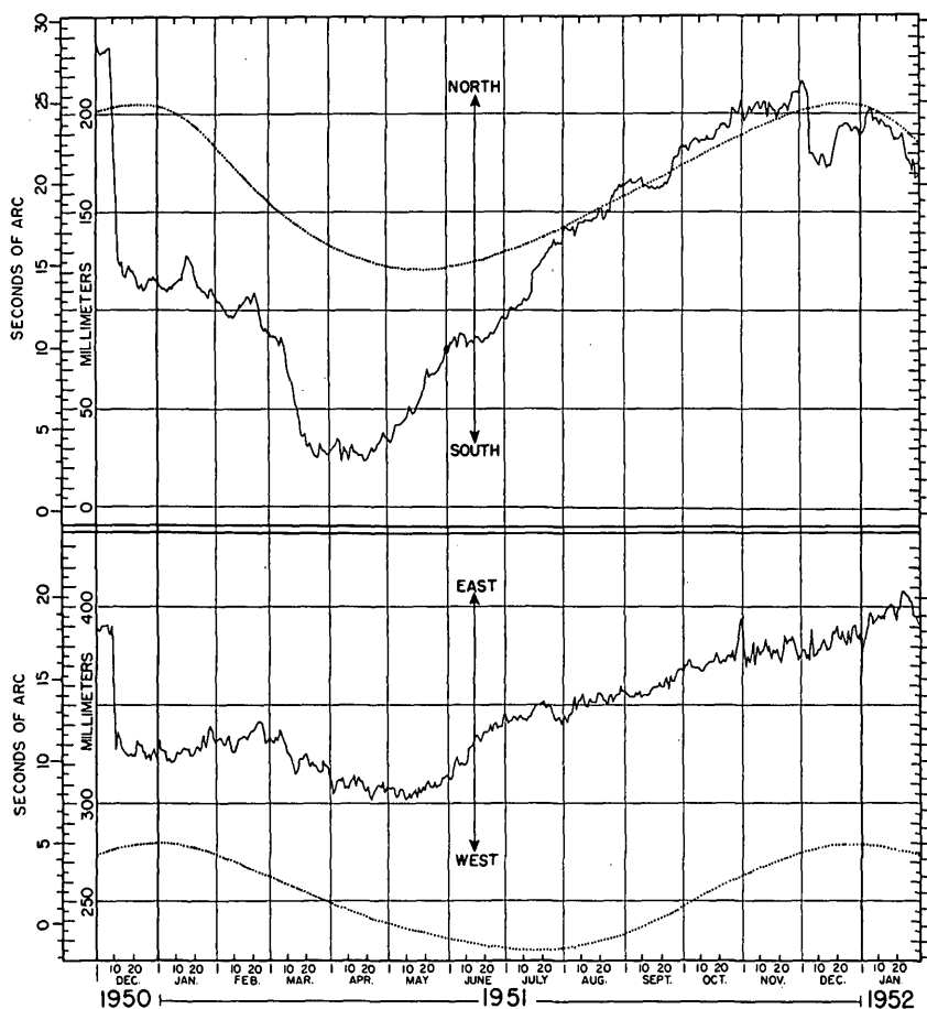
FIGURE 34.—Graph showing ground tilting at the Whitney Laboratory of Seismology, on the northeastern rim of Kilauea caldera, in 1951. The solid line shows the tilt as measured during the year. The dotted line is the approximate normal annual curve for years in which there is no volcanic disturbance.
