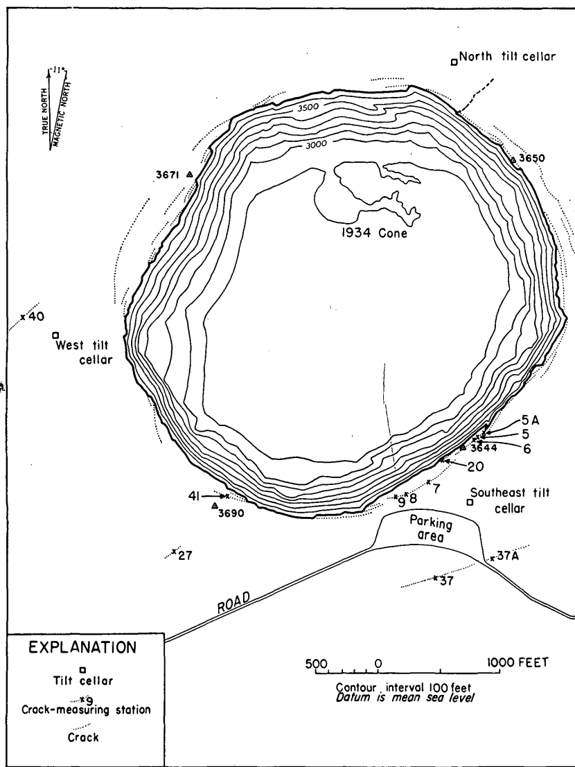
FIGURE 35.—Map of Halemaumau and vicinity, showing the location of tilt-measuring stations and crack-measuring stations.
