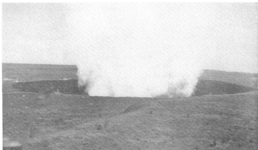
FIGURE 38.—Clouds of steam rising from Halemaumau on October 29, 1951, following heavy rains on the preceding 2 days. The view is from the Hawaiian Volcano Observatory, at Uwekahuna.
