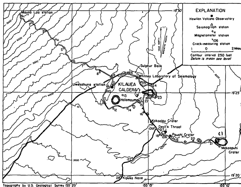
FIGURE 31.—Map showing the location of the Hawaiian Volcano Observatory, seismograph stations, and magnetometer stations, in the vicinity of Kilauea caldera.
