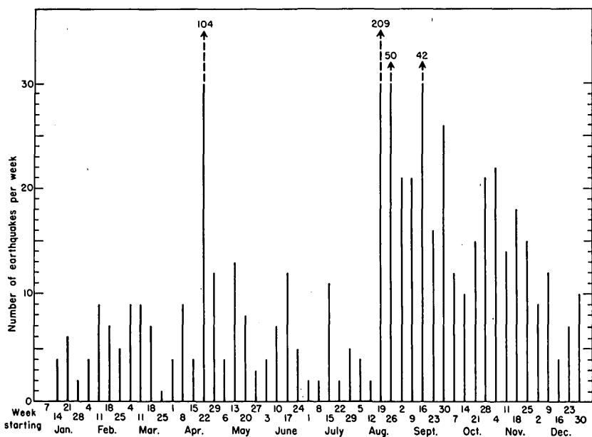
FIGURE 32.—Graph showing the number of earthquakes recorded each week during 1951 at the Whitney Laboratory of Seismology, on the northeastern rim of Kilauea caldera.
