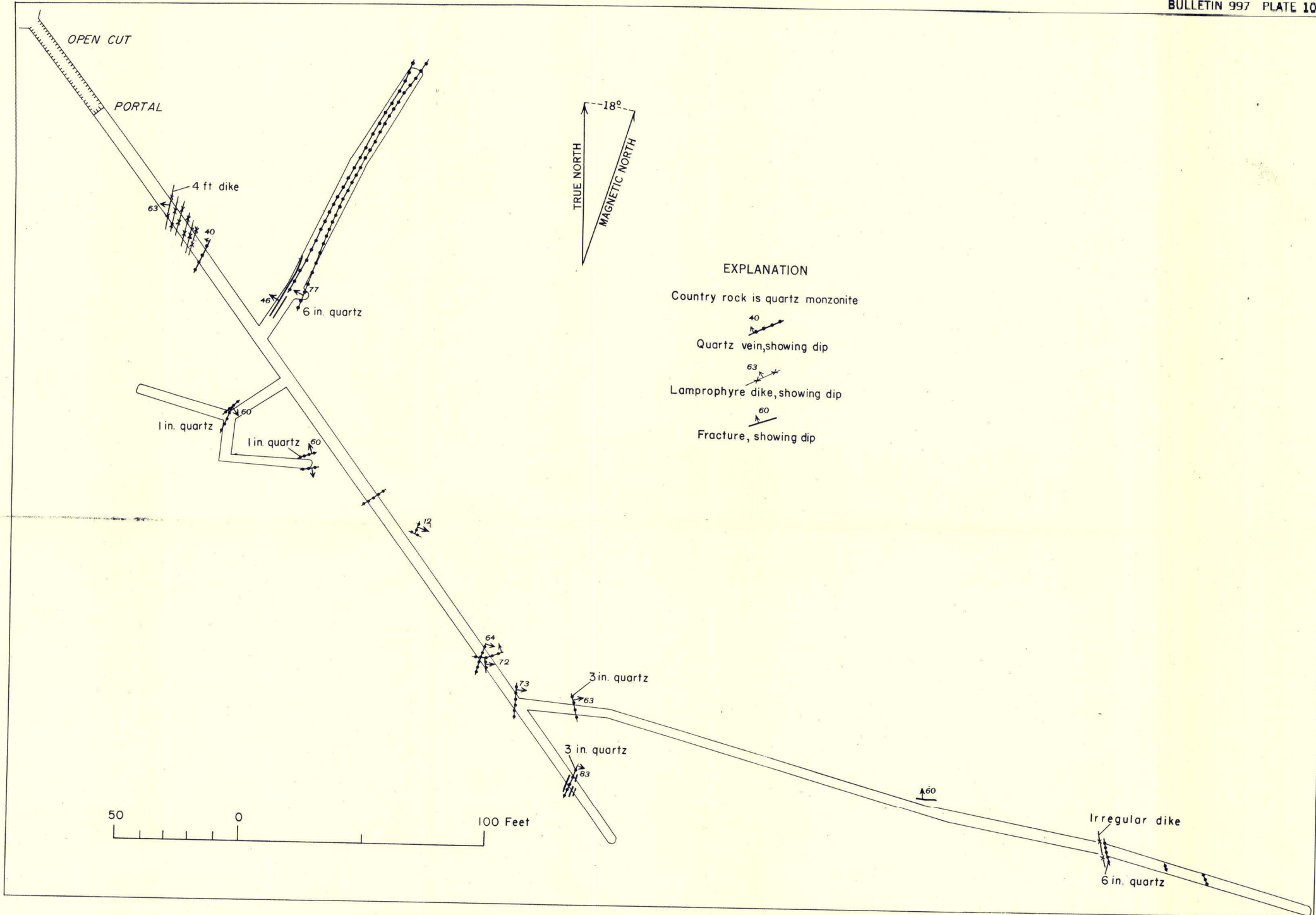
GEOLOGIC SKETCH MAP OF THE CUMMINGS TUNNEL
