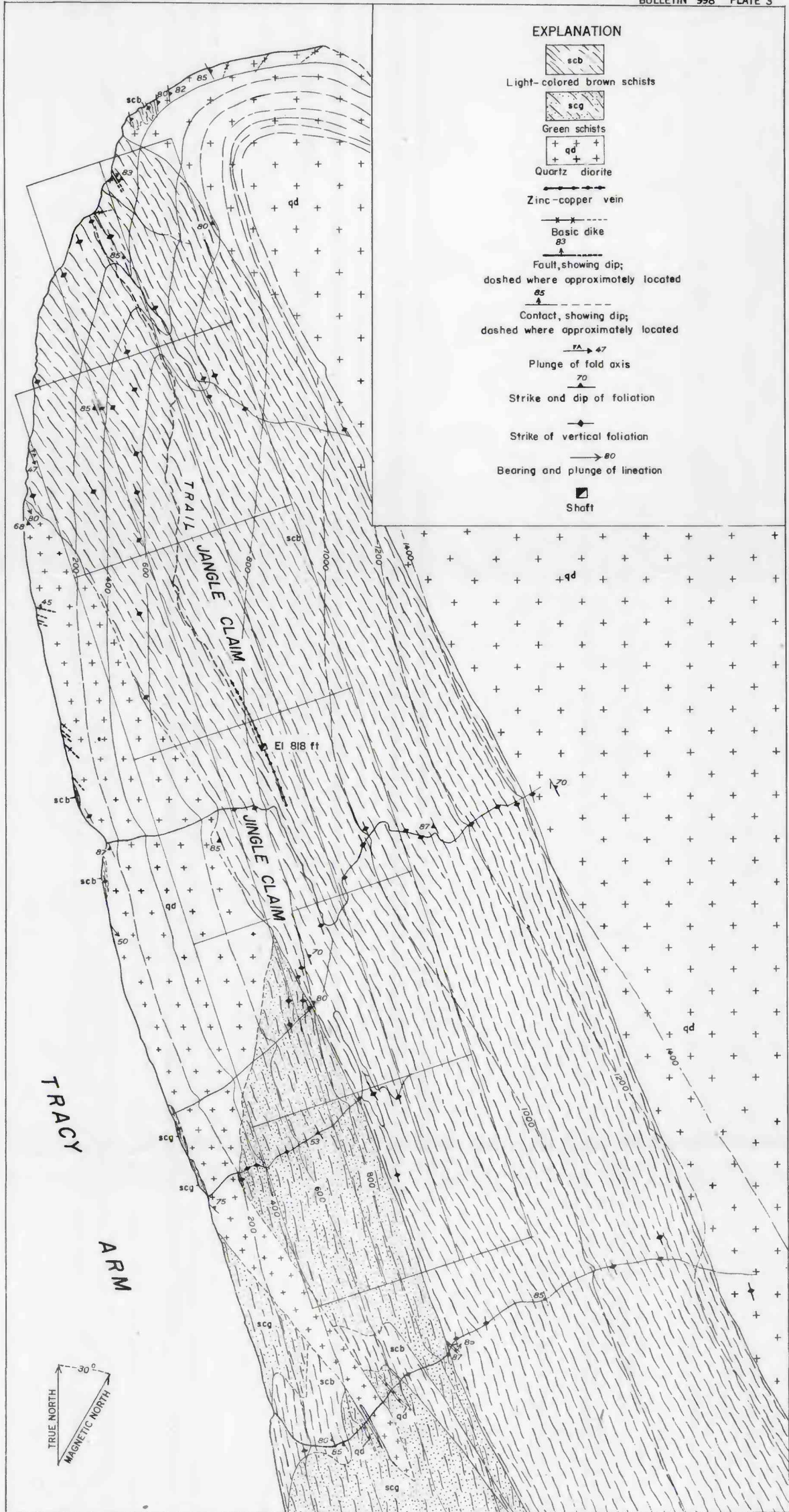
GEOLOGIC MAP OF THE AREA AT THE ELBOW IN TRACY ARM SHOWING LOCATION OF CLAIMS AND POSITION OF THE ZINC-COPPER DEPOSIT
