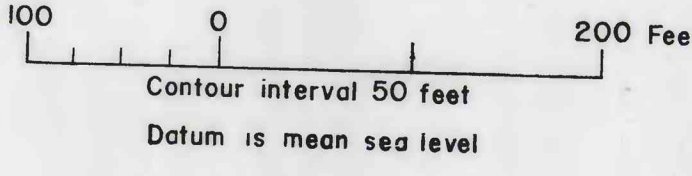
Geology and topography by H.R. Gault and G.M. Flint, Jr., 1943 GEOLOGIC MAP OF THE ZINC-LEAD DEPOSITS AT THE LAKE CLAIMS, WRANGELL DISTRICT, SOUTHEASTERN ALASKA
