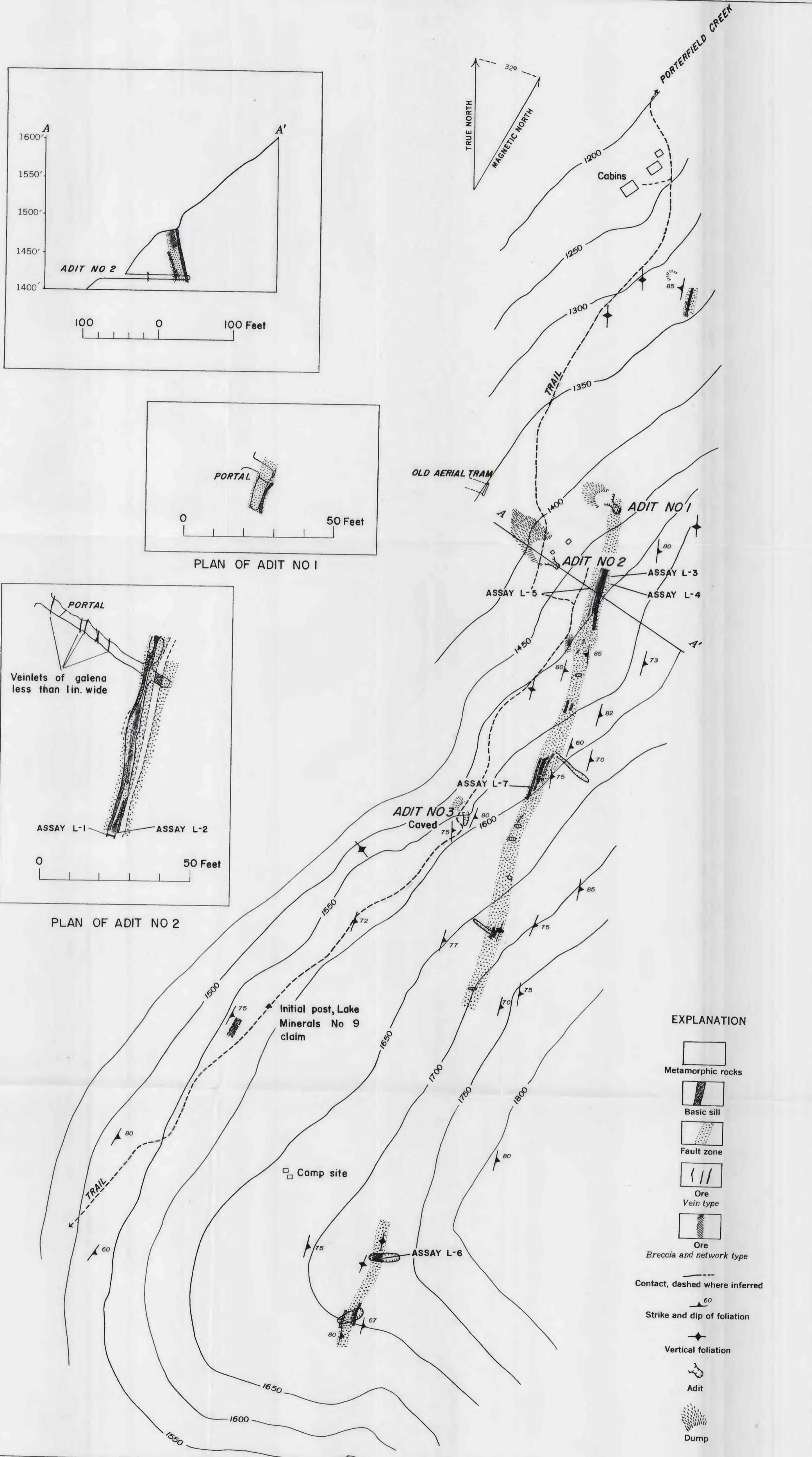
Geology and topography by H.R. Gault and G.M. Flint, Jr., 1943 GEOLOGIC MAP OF THE ZINC-LEAD DEPOSITS AT THE LAKE CLAIMS, WRANGELL DISTRICT, SOUTHEASTERN ALASKA
