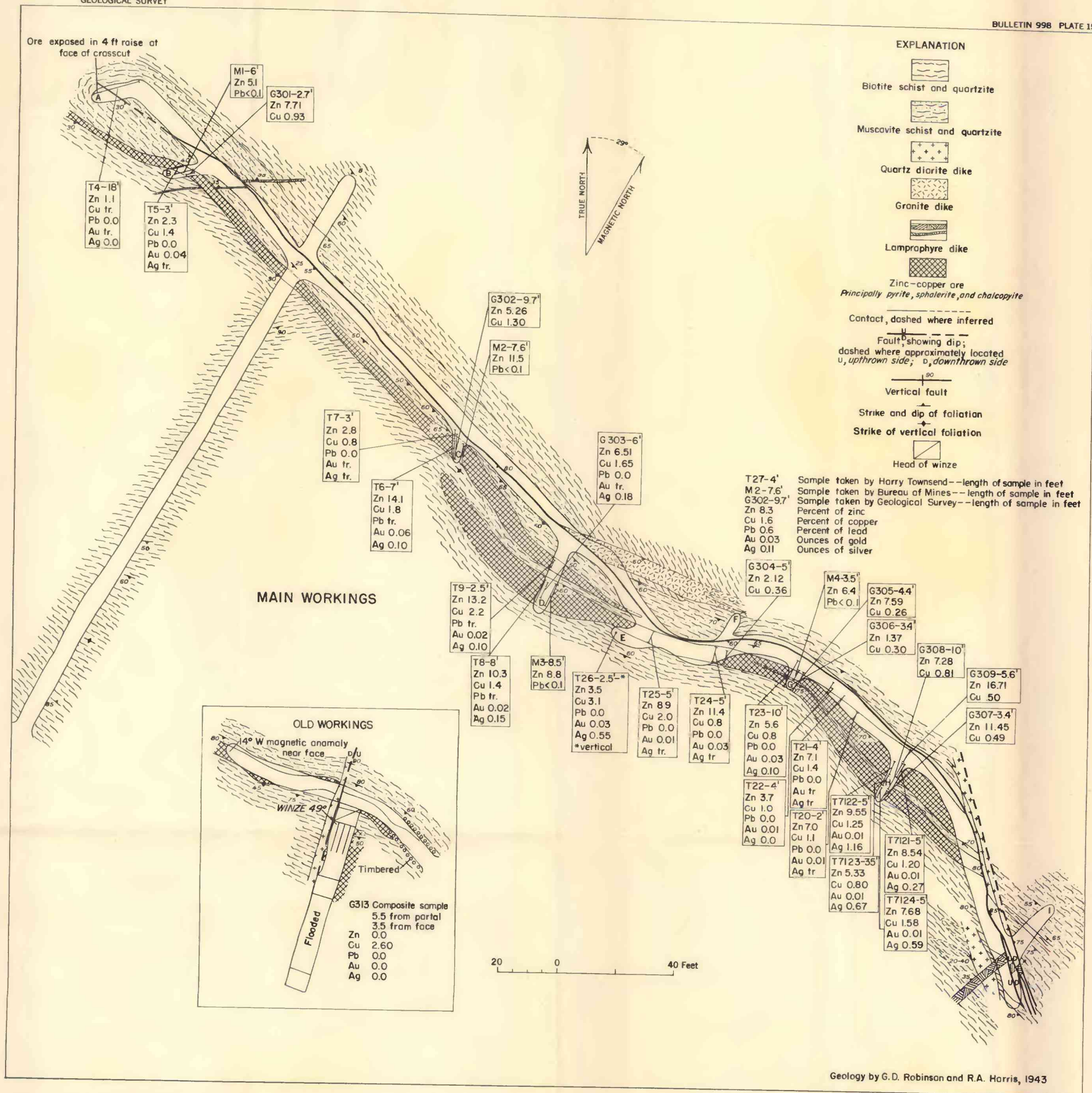
UNDERGROUND WORKINGS OF MOTH BAY ZINC-COPPER DEPOSITS, REVILLAGIGEDO ISLAND, KETCHIKAN DISTRICT, SOUTHEASTERN ALASKA
