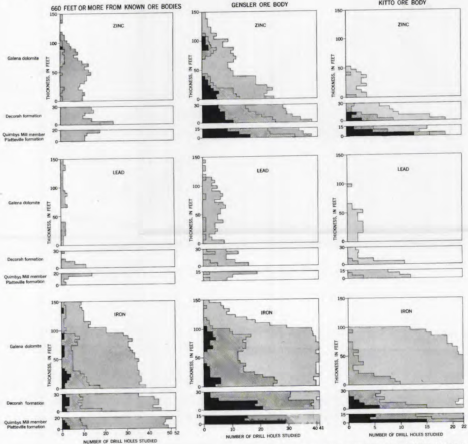
COMPARISON OF MINERALIZATION IN DRILL HOLES CUTTING ORE WITH THAT IN DRILL HOLES NOT NEAR KNOWN ORE, SOUTH OF SHULLSBURG
