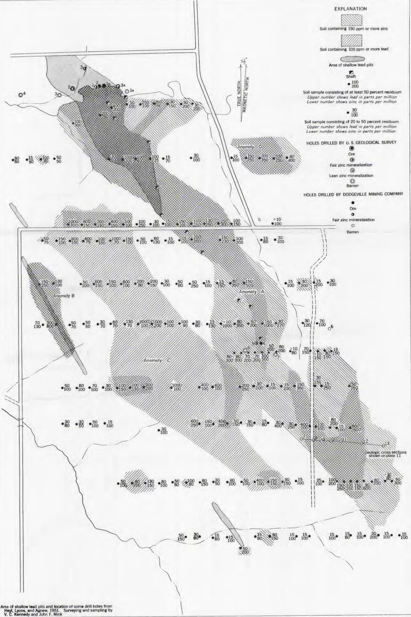
MAP SHOWING LEAD AND ZINC CONTENT OF SOIL, CROW BRANCH AREA
