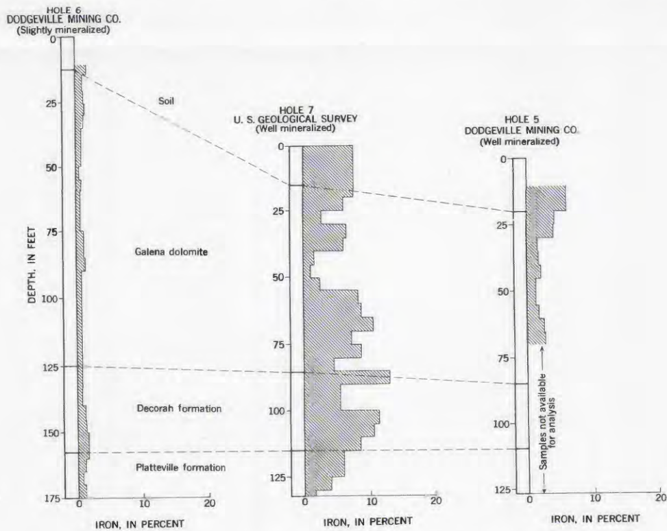
COMPARISON OF ZINC, LEAD, AND IRON CONCENTRATIONS IN A SLIGHTLY-MINERALIZED AREA WITH THOSE OF WELL-MINERALIZED AREAS. CROW BRANCH
