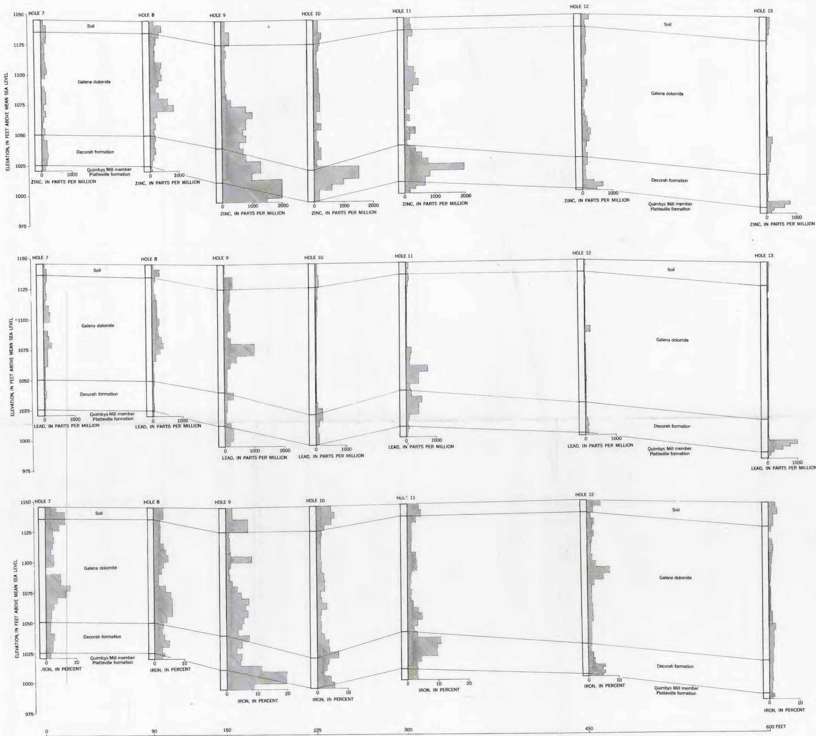
CROSS SECTIONS THROUGH DRILL HOLES 7-13 SHOWING ZINC, LEAD, AND IRON CONCENTRATIONS IN ROCKS AT CROW BRANCH
