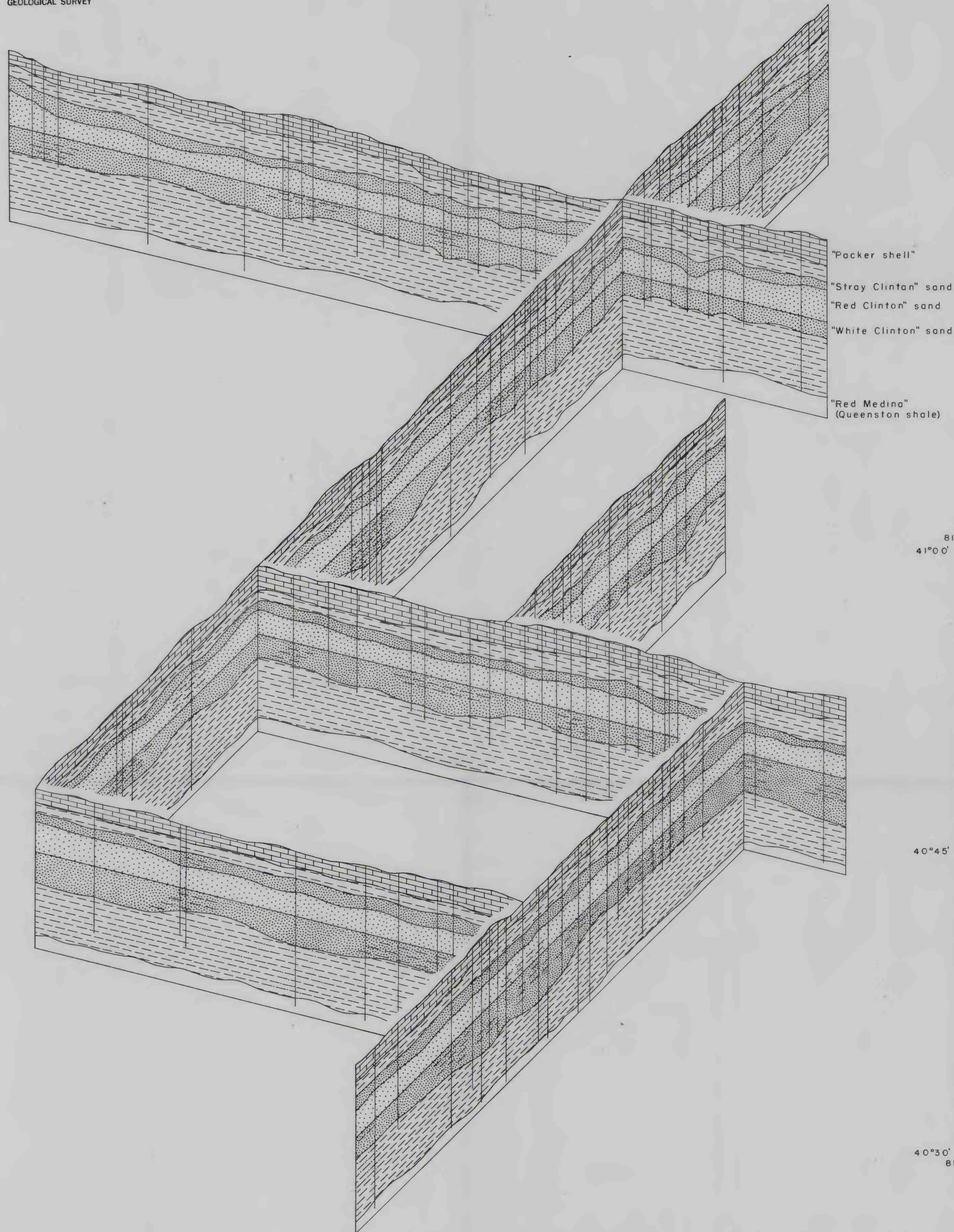
FENCE DIAGRAM OF THE CANTON, DOVER, MASSILLON, AND NAVARRE QUADRANGLES, OHIO, SHOWING THE RELATIONSHIP OF THE THREE "CLINTON" SANDS AND THE RELATIVE POSITION OF THE STRATIGRAPHIC UNITS
