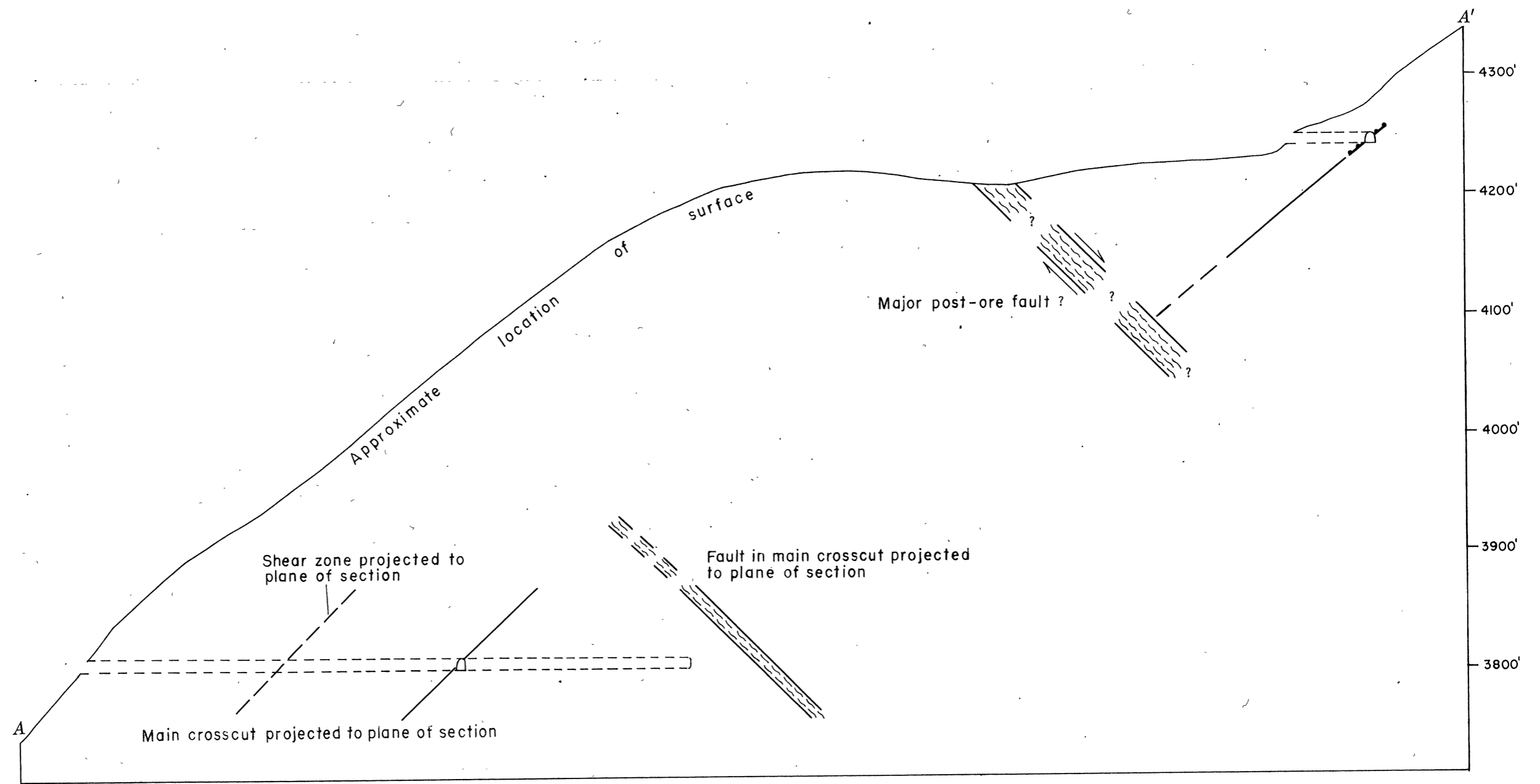
MAP AND SECTION SHOWING UPPER AND LOWER WORKINGS, KELLY-WILLOW PROSPECT
