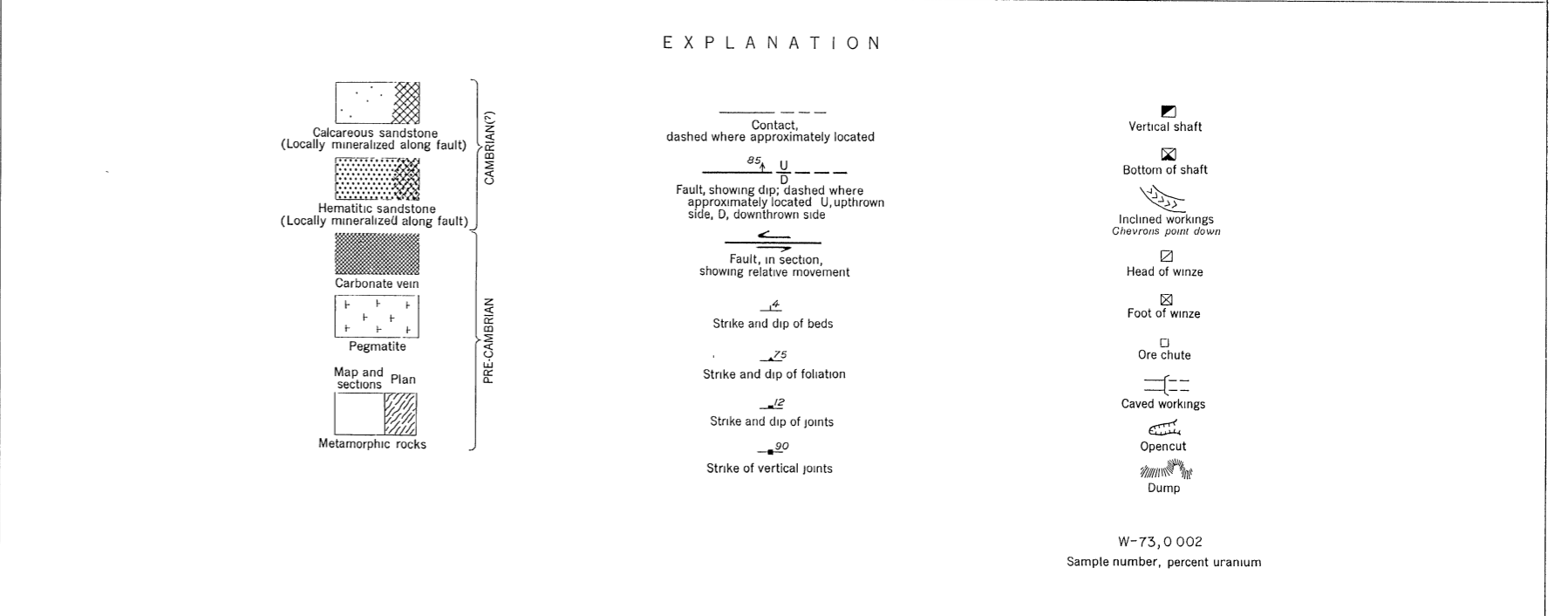
GEOLOGIC MAP, UNDERGROUND WORKINGS, AND SECTIONS OF THE SILVER CLIFF MINE, LUSK, NIOBRARA COUNTY, WYOMING
