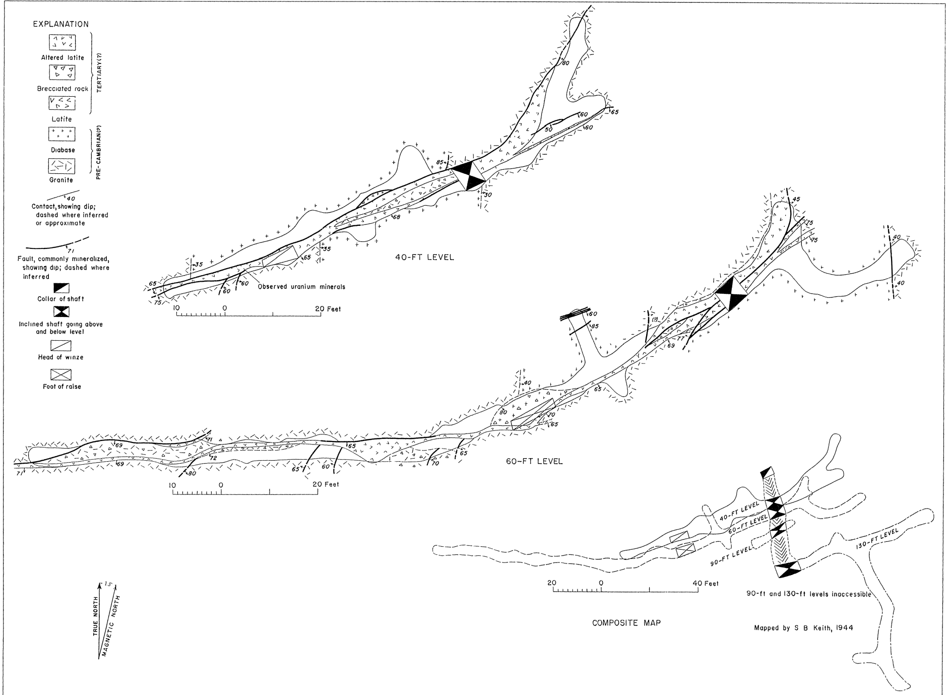
GEOLOGIC MAP, 40-FOOT AND 60-FOOT LEVELS, AND COMPOSITE MAP OF MERRY WIDOW MINE, WHITE SIGNAL DISTRICT, GRANT COUNTY, NEW MEXICO.
