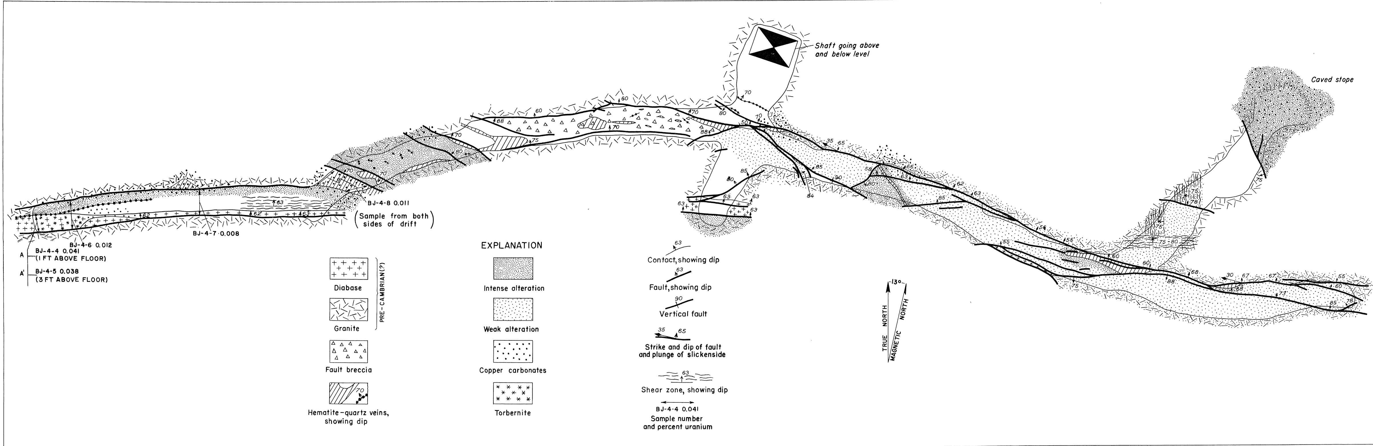
GEOLOGIC MAP, 100-FOOT LEVEL, APACHE TRAIL MINE, GRANT COUNTY, NEW MEXICO.
