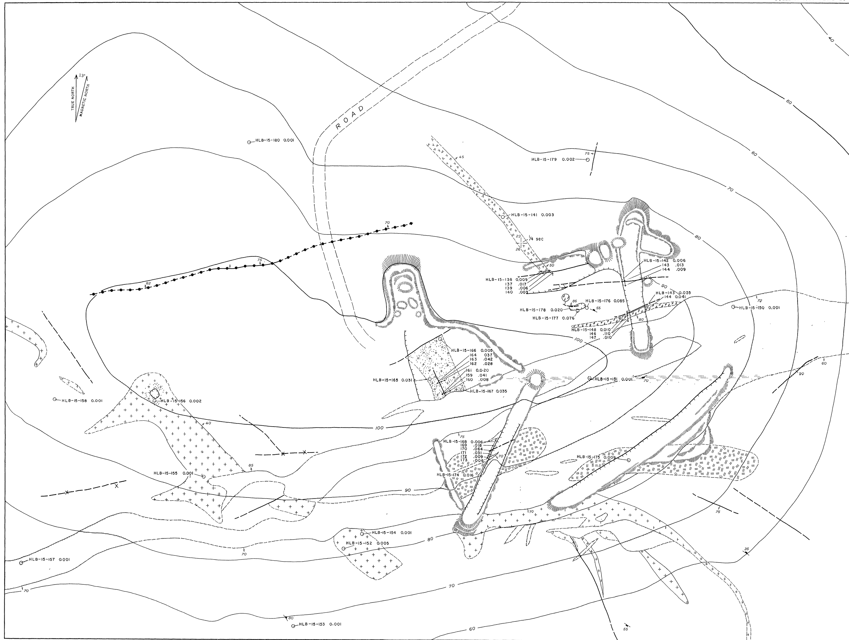
GEOLOGIC MAP AND ASSAY PLAN OF URANIUM OCCURRENCES, BLUE JAY CLAIM, WHITE SIGNAL DISTRICT, GRANT COUNTY, NEW MEXICO
