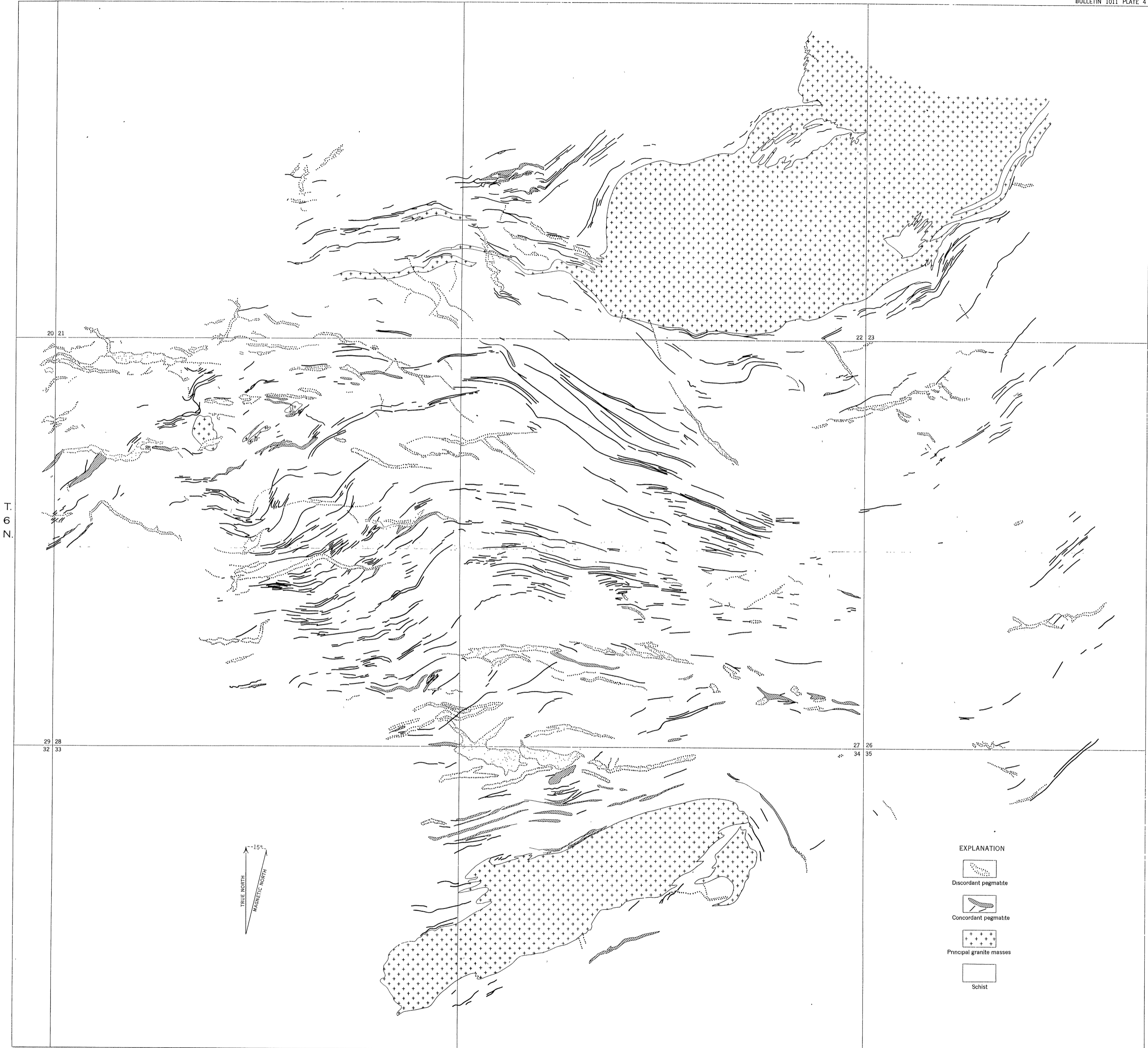
PEGMATITES DISCORDANT IN SCHIST, HYATT AREA, CRYSTAL MOUNTAIN DISTRICT, COLORADO
