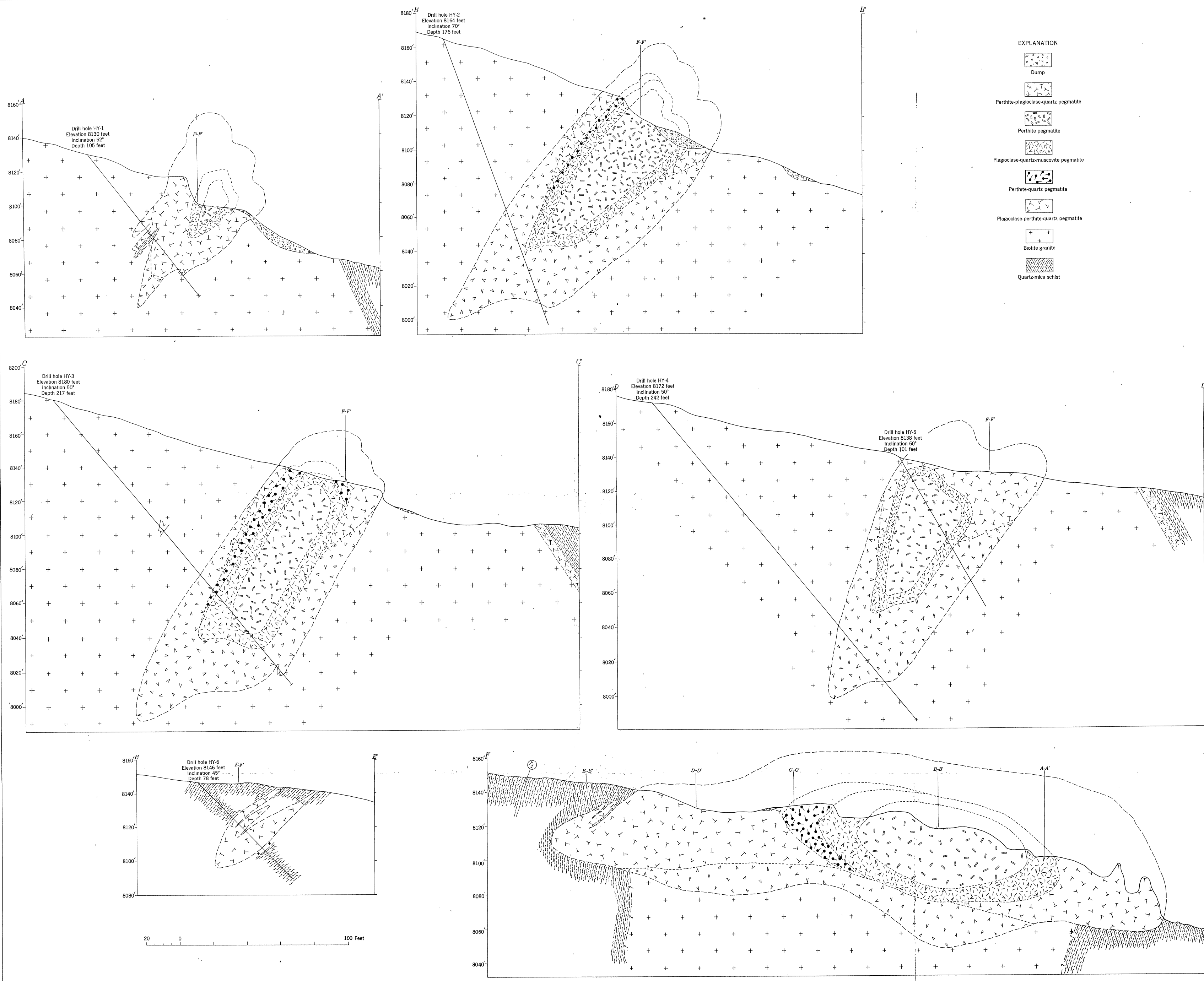
GEOLOGIC CROSS SECTIONS OF THE HYATT PEGMATITE, CRYSTAL MOUNTAIN DISTRICT, COLORADO
