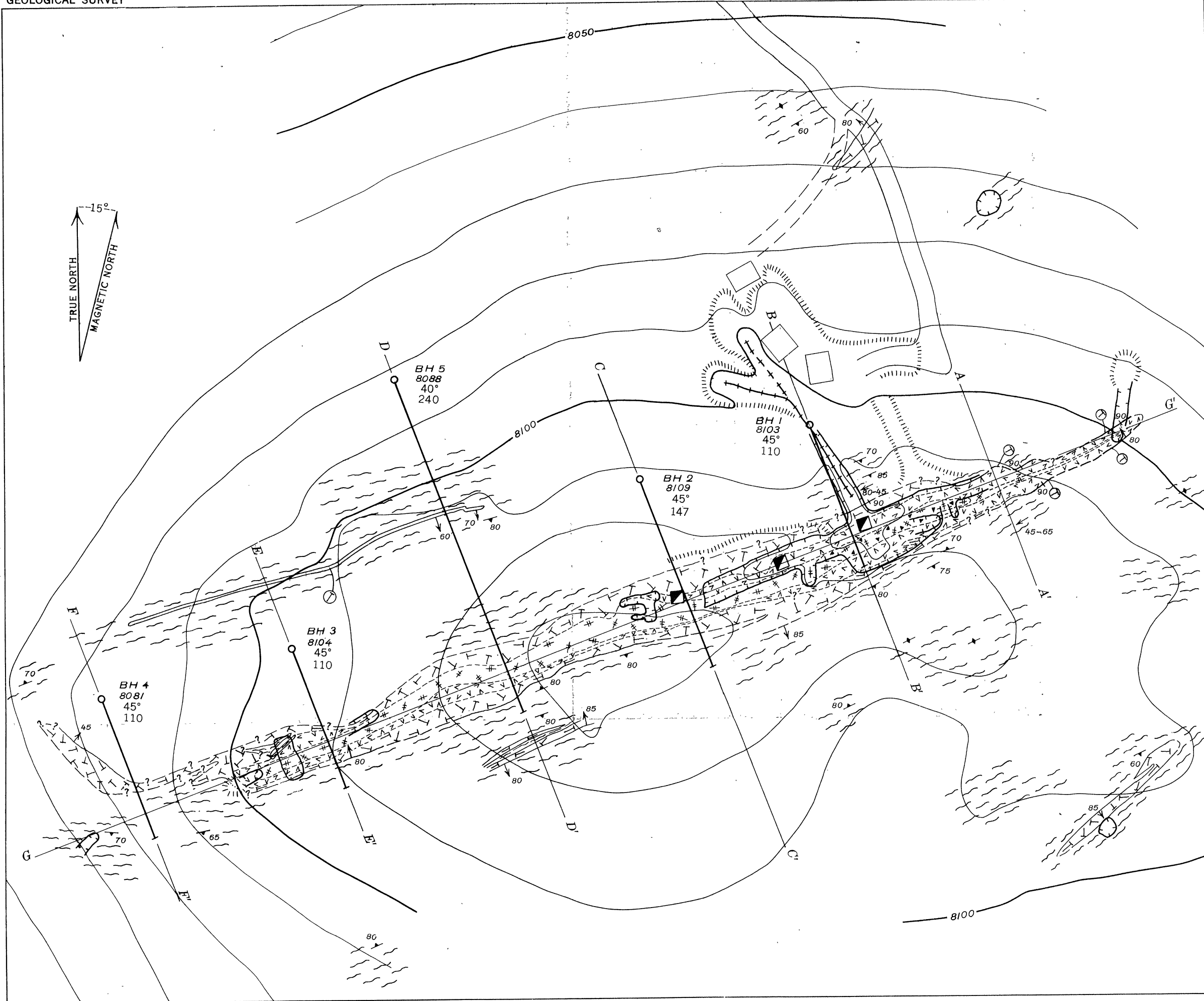
Geology by L.R. Page and J.B. Hanley, Sept. 29-30, 1942 Additions by W.R. Thurston, 1950
