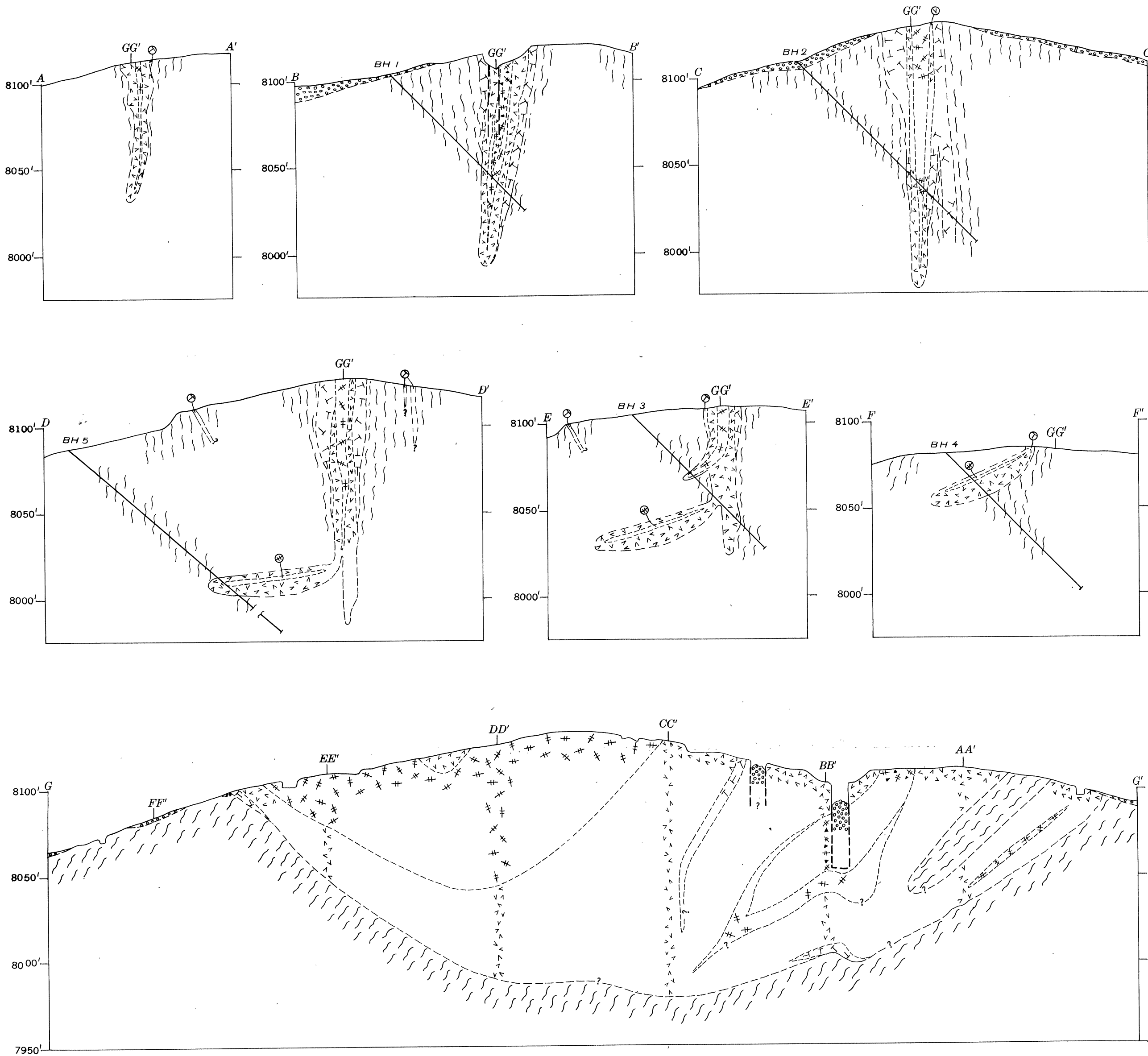
GEOLOGIC MAP AND CROSS SECTIONS OF THE BUCKHORN MICA MINE, CRYSTAL MOUNTAIN DISTRICT, COLORADO
