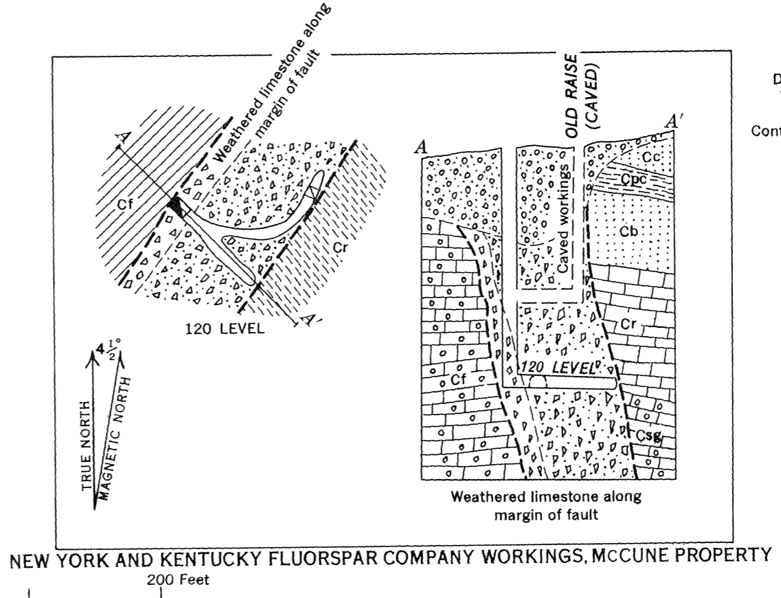
MAPS AND SECTIONS OF SOME WORKINGS OF THE TIGHTWAD (L. E. WADDELL), MCCUNE, AND LA RUE (RIGGS) PROPERTIES, MOORE HILL FAULT SYSTEM
