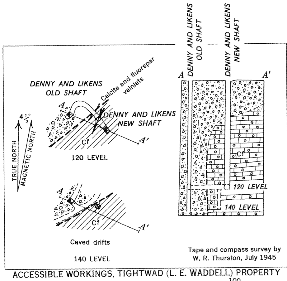
MAPS AND SECTIONS OF SOME WORKINGS OF THE TIGHTWAD (L. E. WADDELL), MCCUNE, AND LA RUE (RIGGS) PROPERTIES, MOORE HILL FAULT SYSTEM
