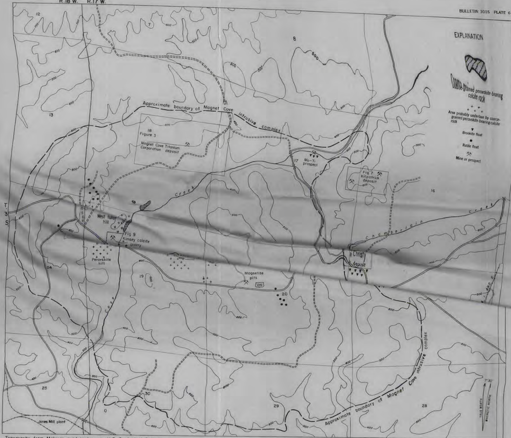
TOPOGRAPHIC MAP OF MAGNET COVE, HOT SPRINGS COUNTY ARKANSAS, SHOWING THE LOCATION OF KNOWN DEPOSITS OF RUTILE AND BROOKITE
