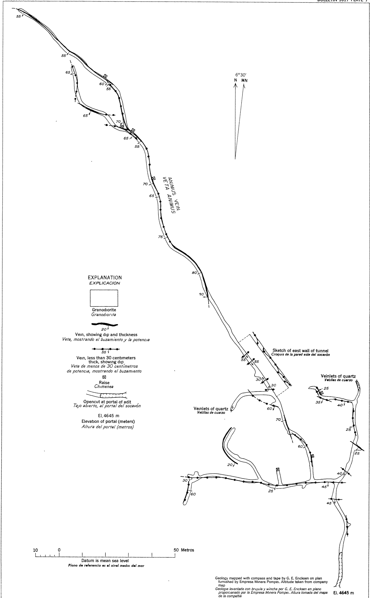
GEOLOGIC MAP OF THE SANTA RITA LEVEL, HUAMANA MINE QUEBRADA HONDA-VESUVIO MINING DISTRICT, PERU MAPA GEOLOGICO DEL NIVEL SANTA RITA, MINA HUAMANA, DISTRITO MINERO QUEBRADA HONDA-VESUVIO
