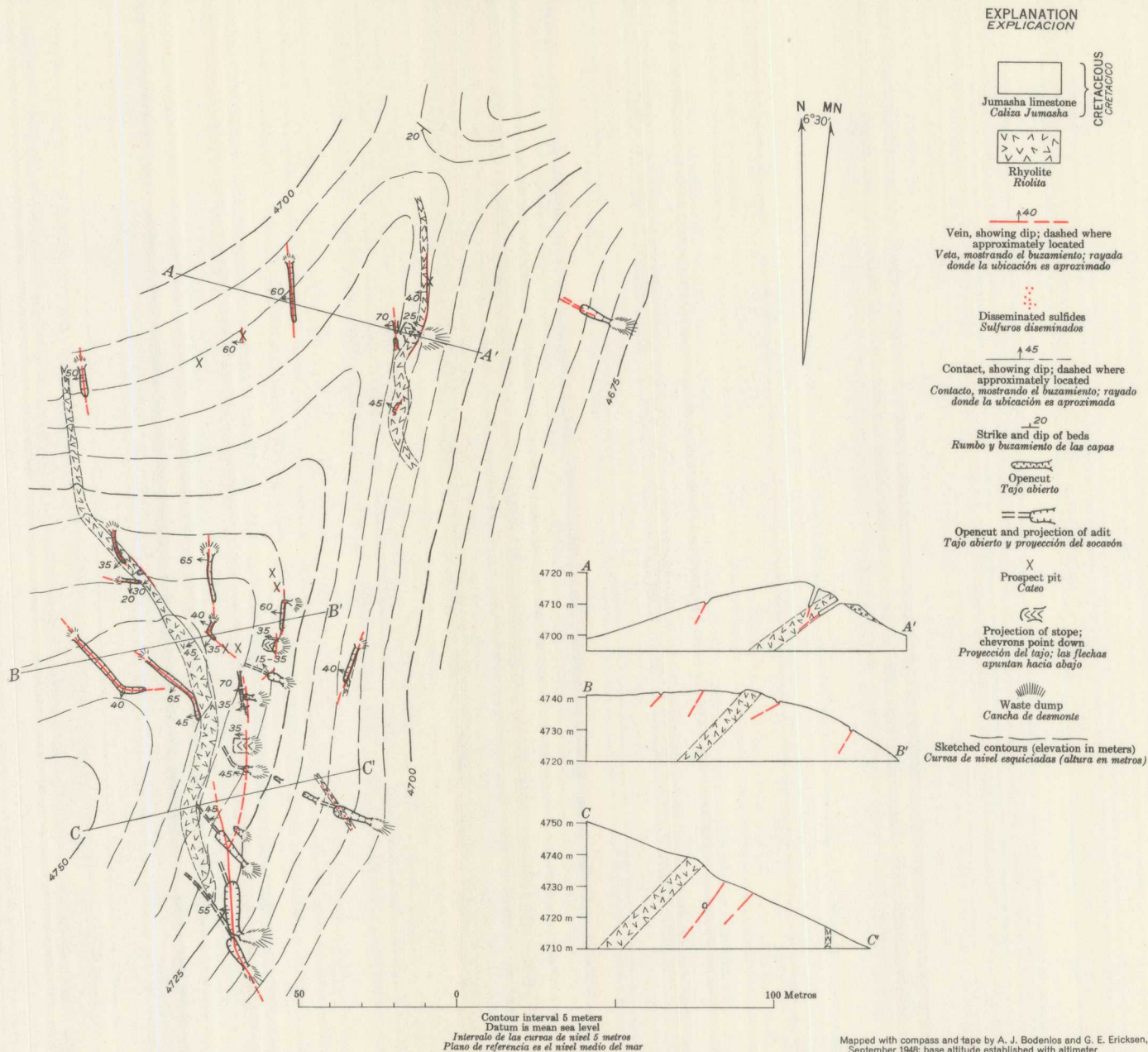
GEOLOGIC SKETCH MAP AND SECTIONS OF THE FORTUNA MINE, ANTAMINA-CONTONGA MINING DISTRICT, PERU CROQUIS GEOLOGICO Y PERFILES DE LA MINA FORTUNA, DISTRITO MINERO DE ANTAMINA-CONTONGA
