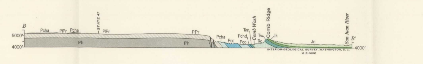
GEOLOGIC MAP AND SECTIONS OF COMB RIDGE AND VICINITY NORTH OF SAN JUAN RIVER, SAN JUAN COUNTY, UTAH
